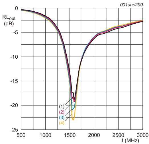
V_{CC} = 1.8 \text{ V} ; P_i = -45 \text{ dBm} . (1) T_{\text{amb}} = -40 \text{ }^\circ\text{C} (2) T_{\text{amb}} = +25 \text{ }^\circ\text{C} (3) T_{\text{amb}} = +85 \text{ }^\circ\text{C} (4) T_{\text{amb}} = +125 \text{ }^\circ\text{C}
