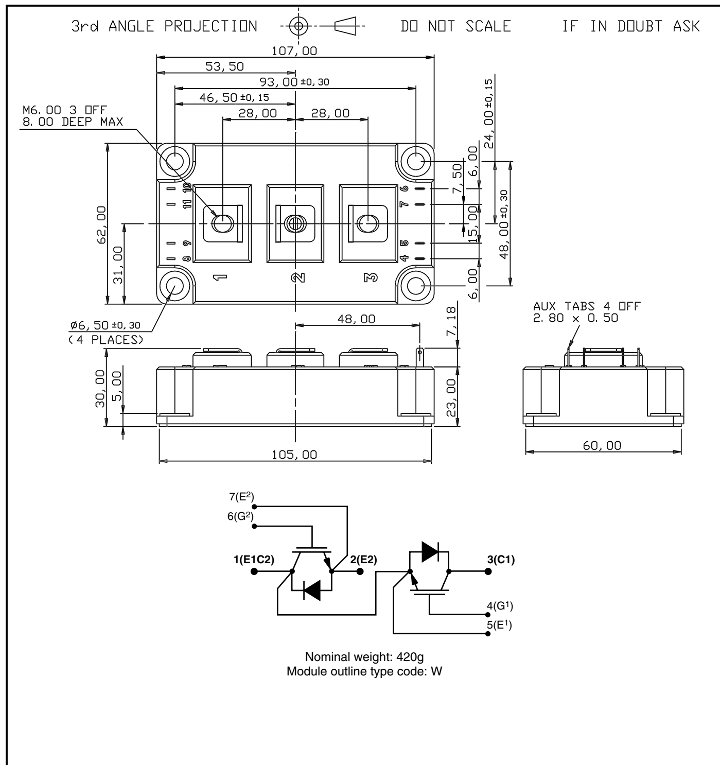
Fig. 6 Package details
