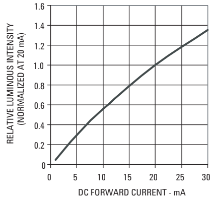
Figure 5. Relative intensity vs. DC forward current.
