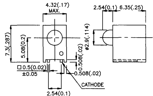
T-1 (3mm) Right Angle
