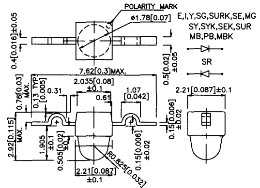
Subminiature Solid State Lamps Z-Bend Lead
