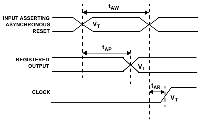
Asynchronous Reset
