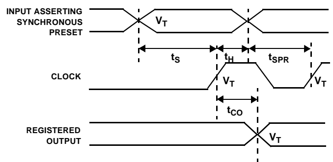
Synchronous Preset
