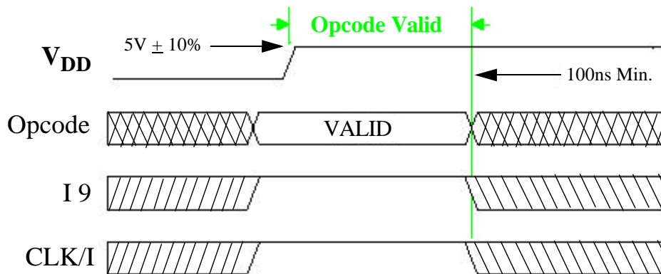
Figure 1. Opcode Timing
