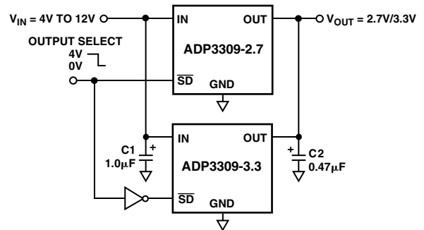
Figure 3. Crossover Switch
