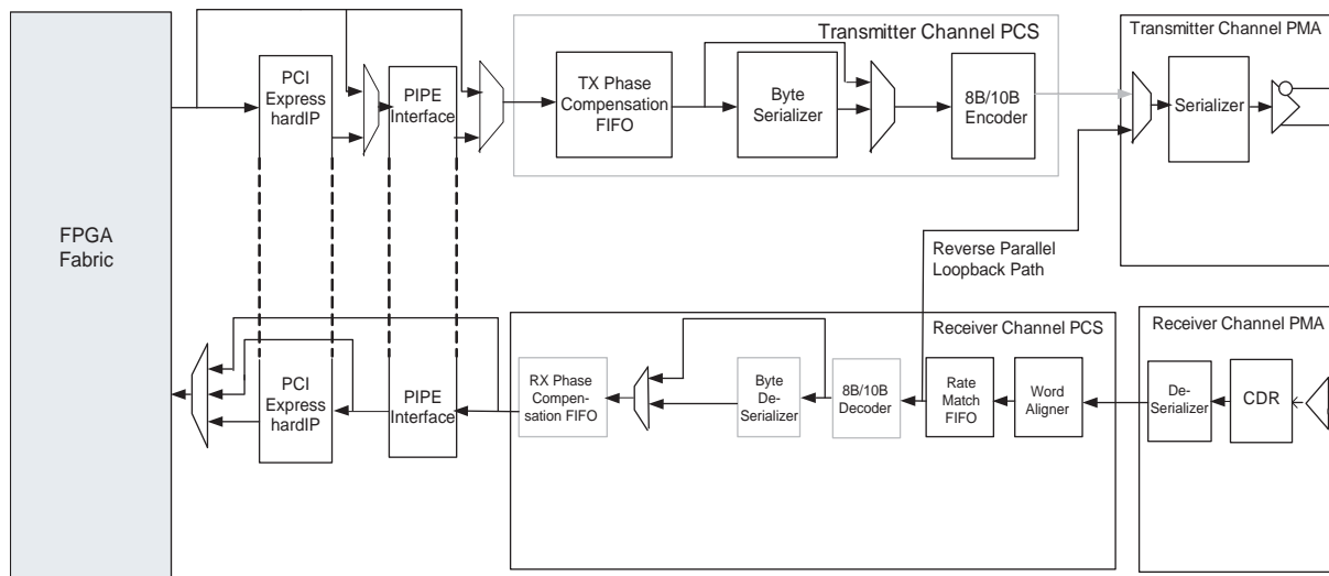
Figure 1-112. PCI Express (PIPE) Reverse Parallel Loopback Mode Datapath
