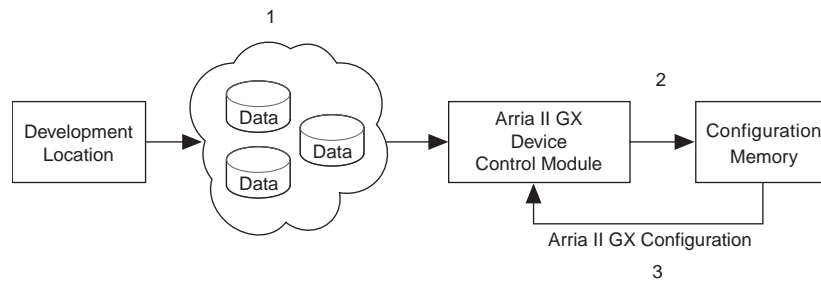
Figure 9-21. Functional Diagram of Arria II GX Remote System Upgrade
