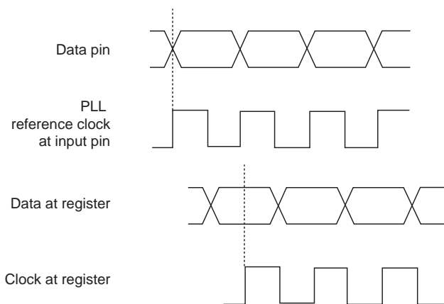
Figure 5-16. Source-Synchronous Mode for LVDS Compensation
