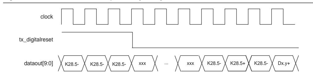
Figure 1-20. 8B/10B Encoder Output during tx\_digitalreset Assertion
