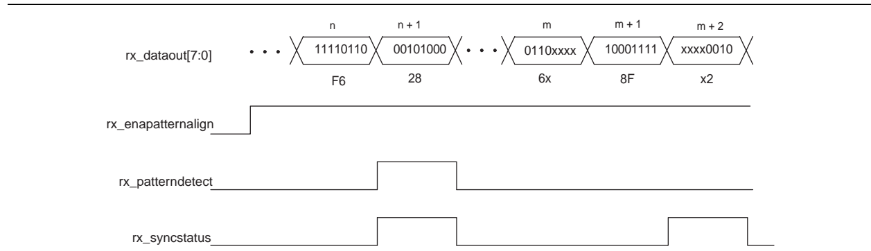
Figure 1-43. Bit-Slip Mode in 8-Bit PMA-PCS Interface Mode
