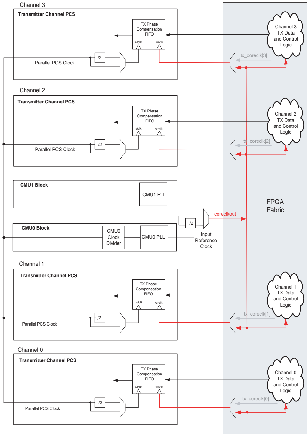
Figure 2-18. FPGA Fabric-Transmitter Interface Clocking in an ×4 Bonded Channel Configuration
