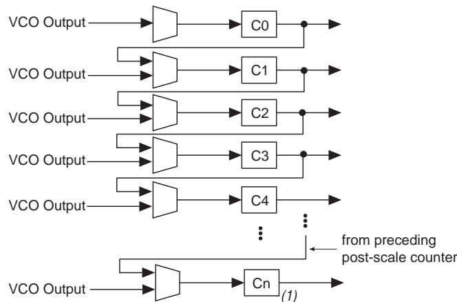
Figure 5-20. Counter Cascading
