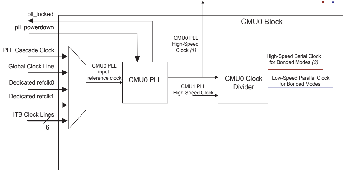
Figure 1-8. Diagram of CMU0 Block
