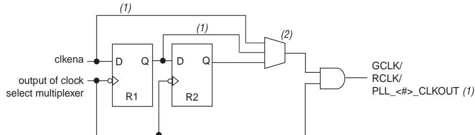
Figure 5-10. clkena Implementation
