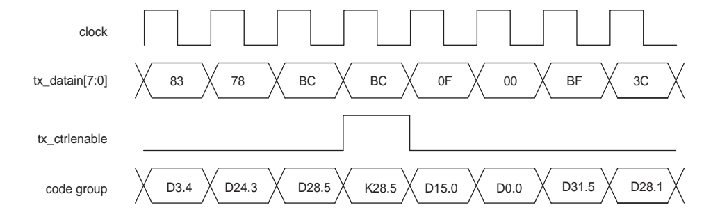
Figure 1-19. Control Word and Data Word Transmission
