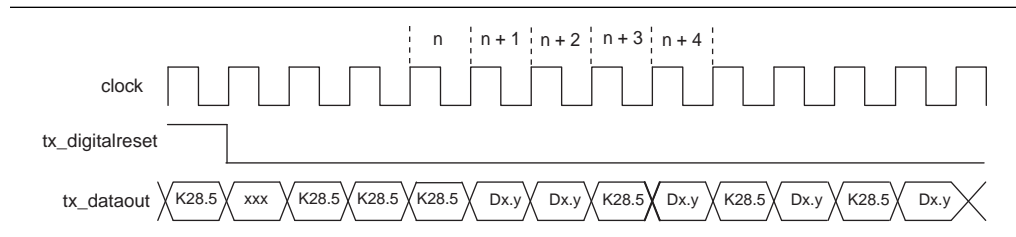
Figure 1-95. Example of Reset Condition in GIGE Mode
