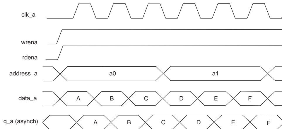
Figure 3-14. Same Port Read-During Write: New Data Mode
