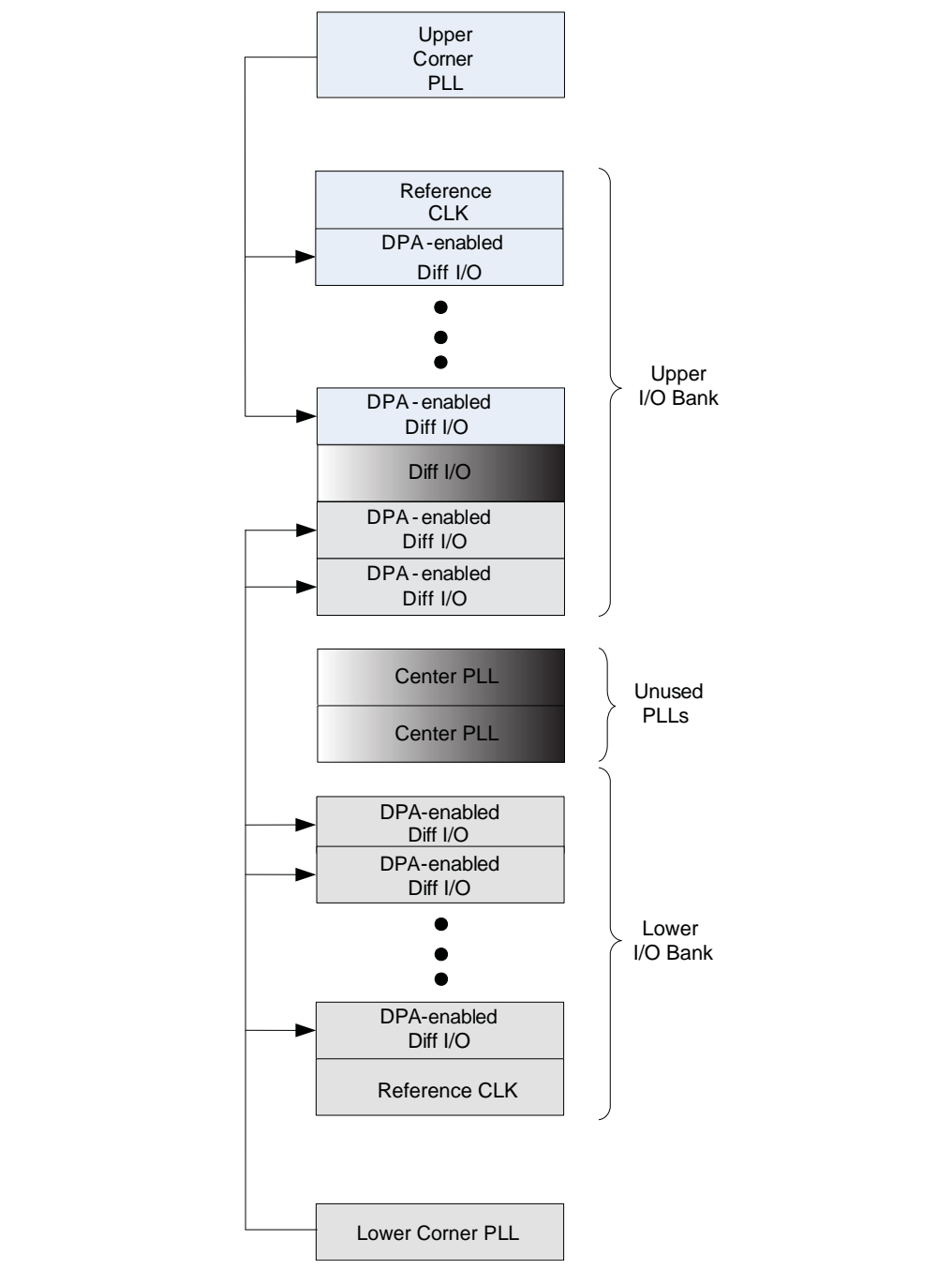
Figure 8-24. Corner PLLs Driving DPA-Enabled Differential I/Os
