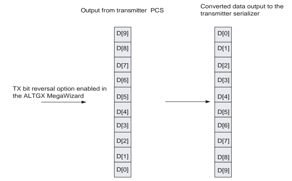
Figure 1–23. Transmitter Bit Reversal Operation in Basic Single-Width Mode
