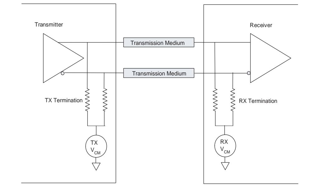
Figure 1-32. DC-Coupled Link
