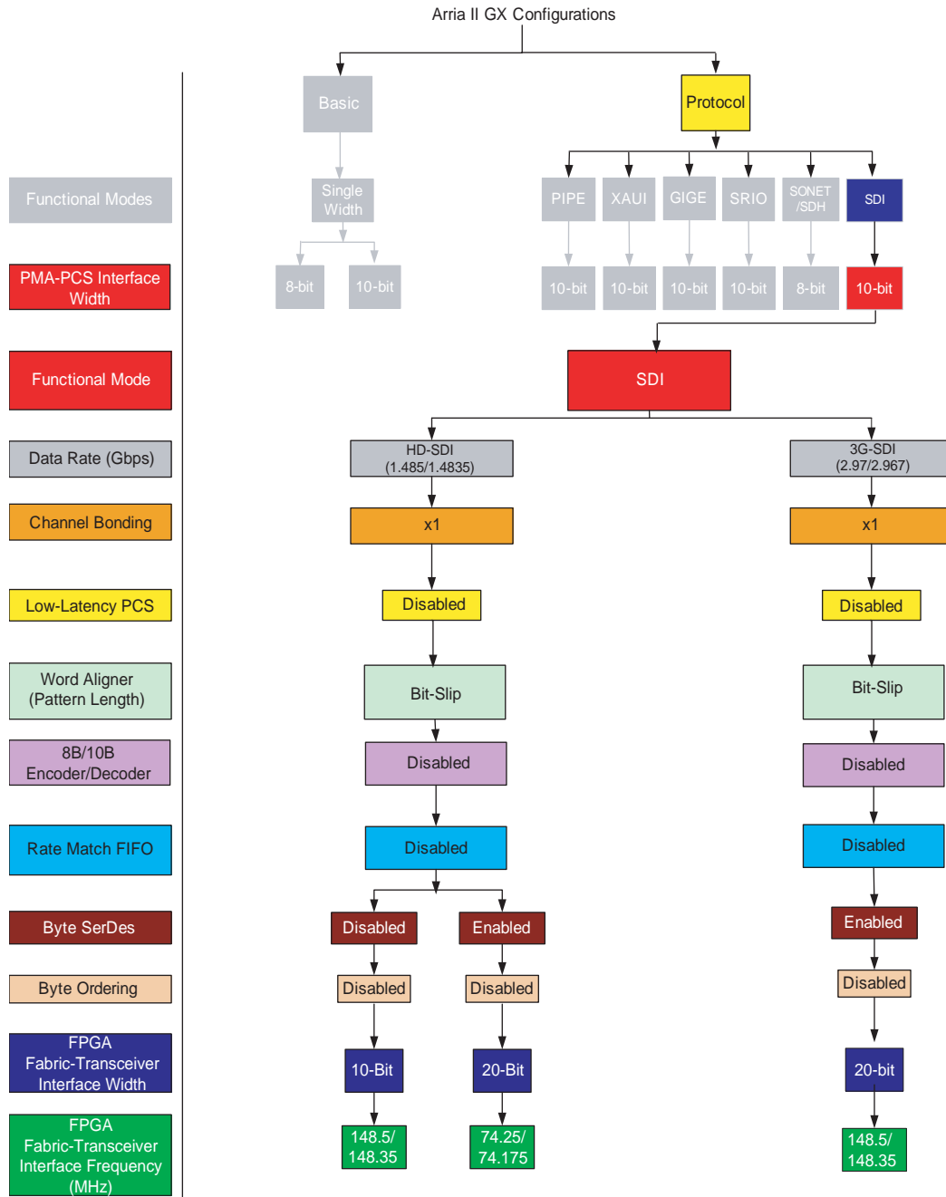
Figure 1-104. SDI Mode
