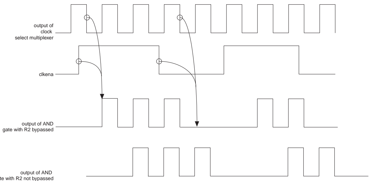
Figure 5-11. clkena Signals
