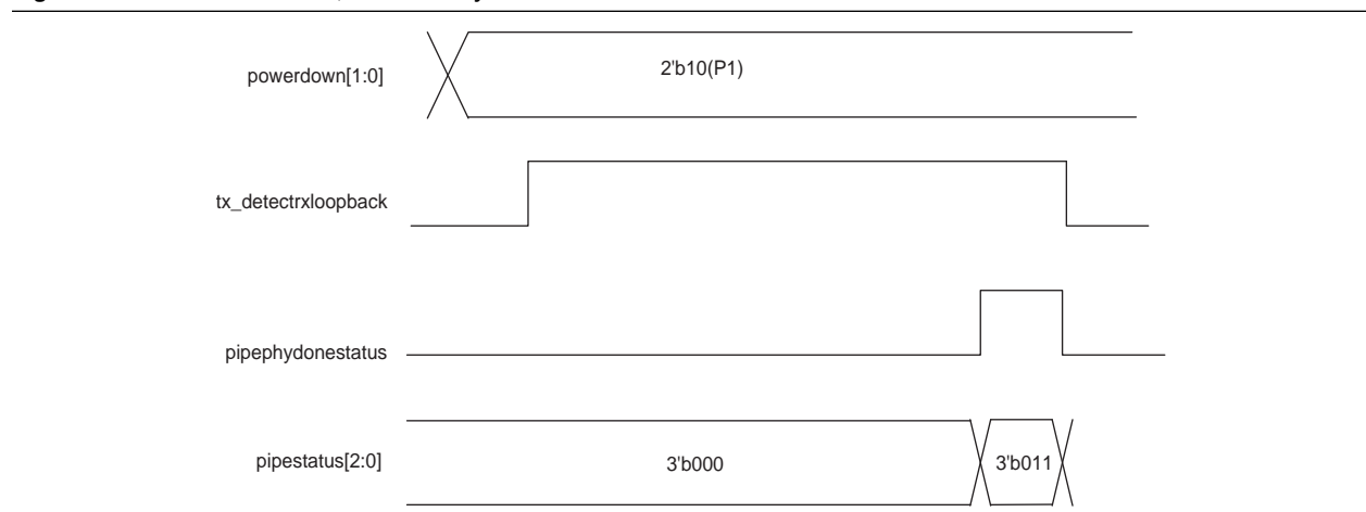
Figure 1-75. Receiver Detect, Successfully Detected
