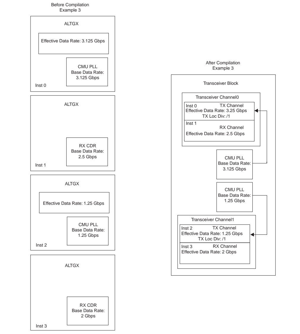
Figure 3-3. ALTGX Transceiver Channel Instances before and after Compilation for Example 3
