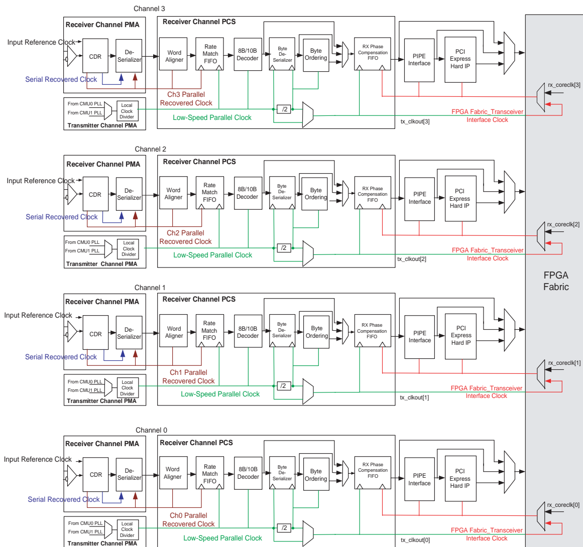
Figure 2-12. Receiver Datapath Clcking in Non-Bonded Configurations with Rate Matcher
