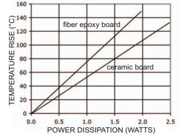
POWER DISSIPATION
