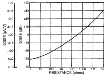
CURRENT NOISE
