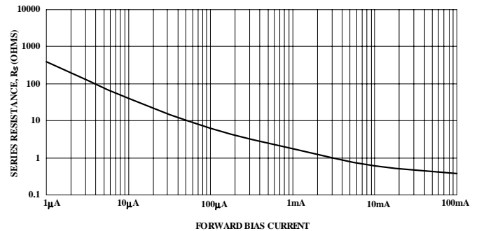
Resistance vs Forward Current (MA4P789 Series)
