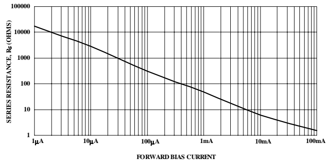
Resistance vs Forward Current (MA4P278 Series)
