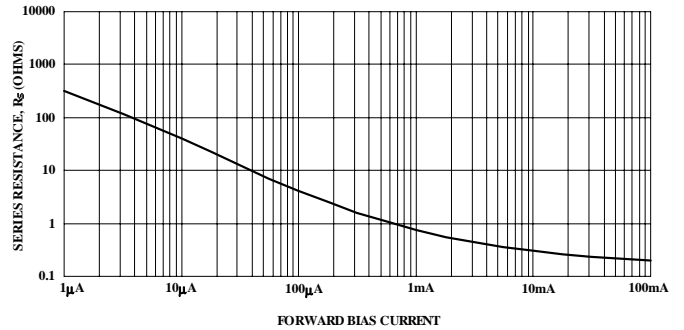
Resistance vs Forward Current (MA4P275 Series)
