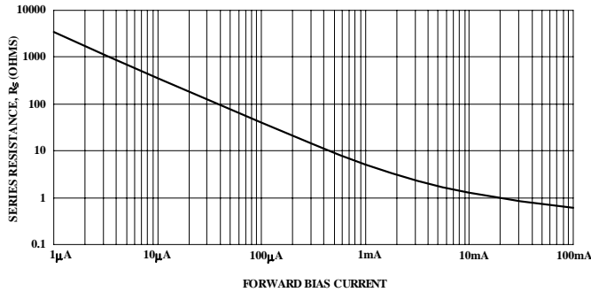
Resistance vs Forward Current (MA4P274 Series)
