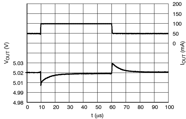
Figure 32. Load Transients, 5.0 V Version, I_{OUT} = 50 - 100 \text{ mA} , t_R = t_F = 0.5 \text{ } \mu\text{s} , V_{IN} = 6.0 \text{ V}
