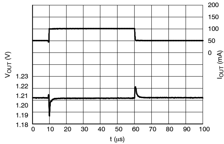
Figure 30. Load Transients, 1.2 V Version, I_{OUT} = 50 - 100 \text{ mA} , t_R = t_F = 0.5 \text{ } \mu\text{s} , V_{IN} = 2.2 \text{ V}
