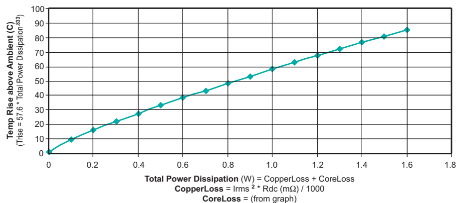
Temp Rise vs Power Dissipation
