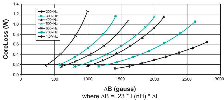
CoreLoss vs Flux Density
