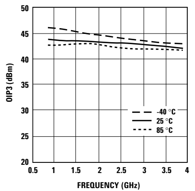
Figure 16. OIP3 vs. Temp and Freq.
