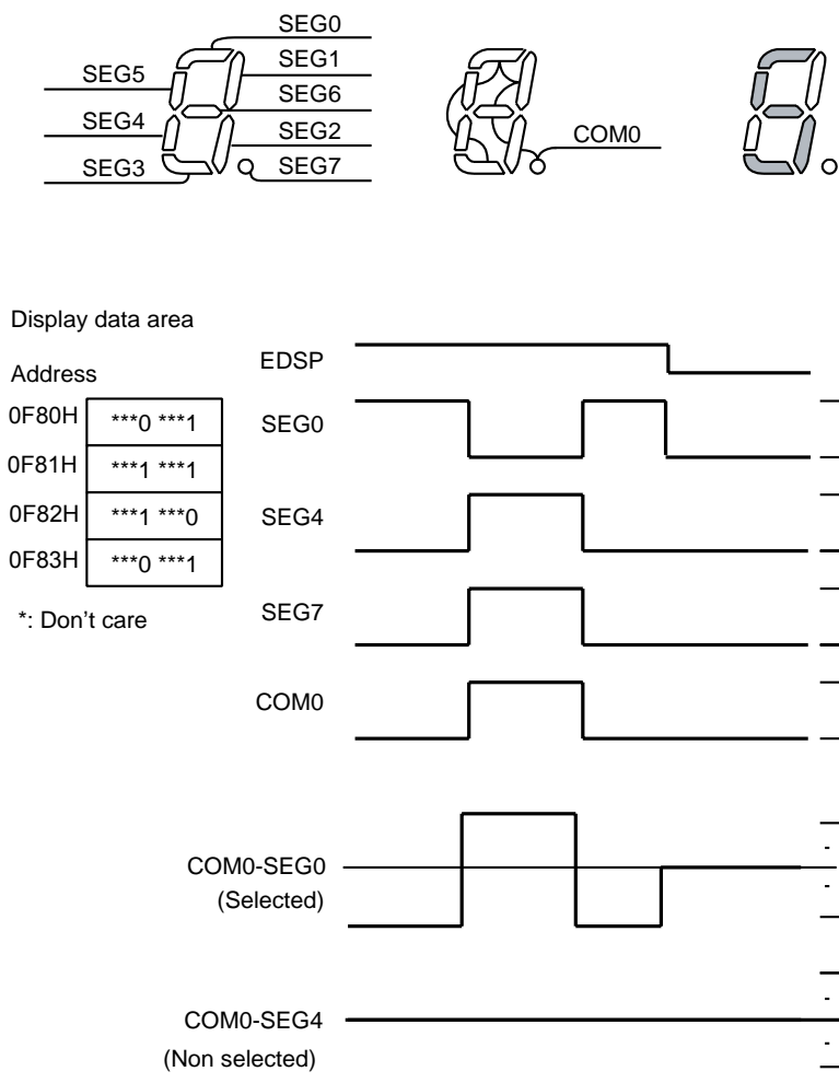
Figure 13-11 Static Drive
