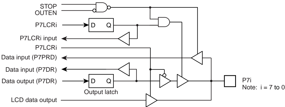
Figure 5-7 Port 7
