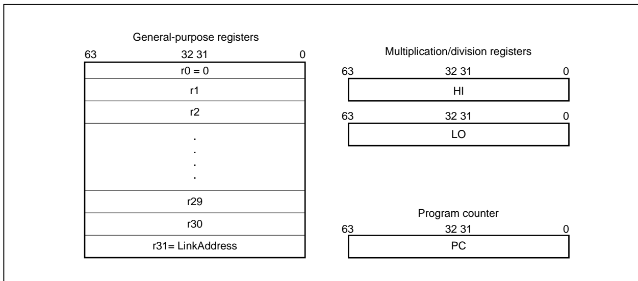
Figure 3-2. CPU Registers
