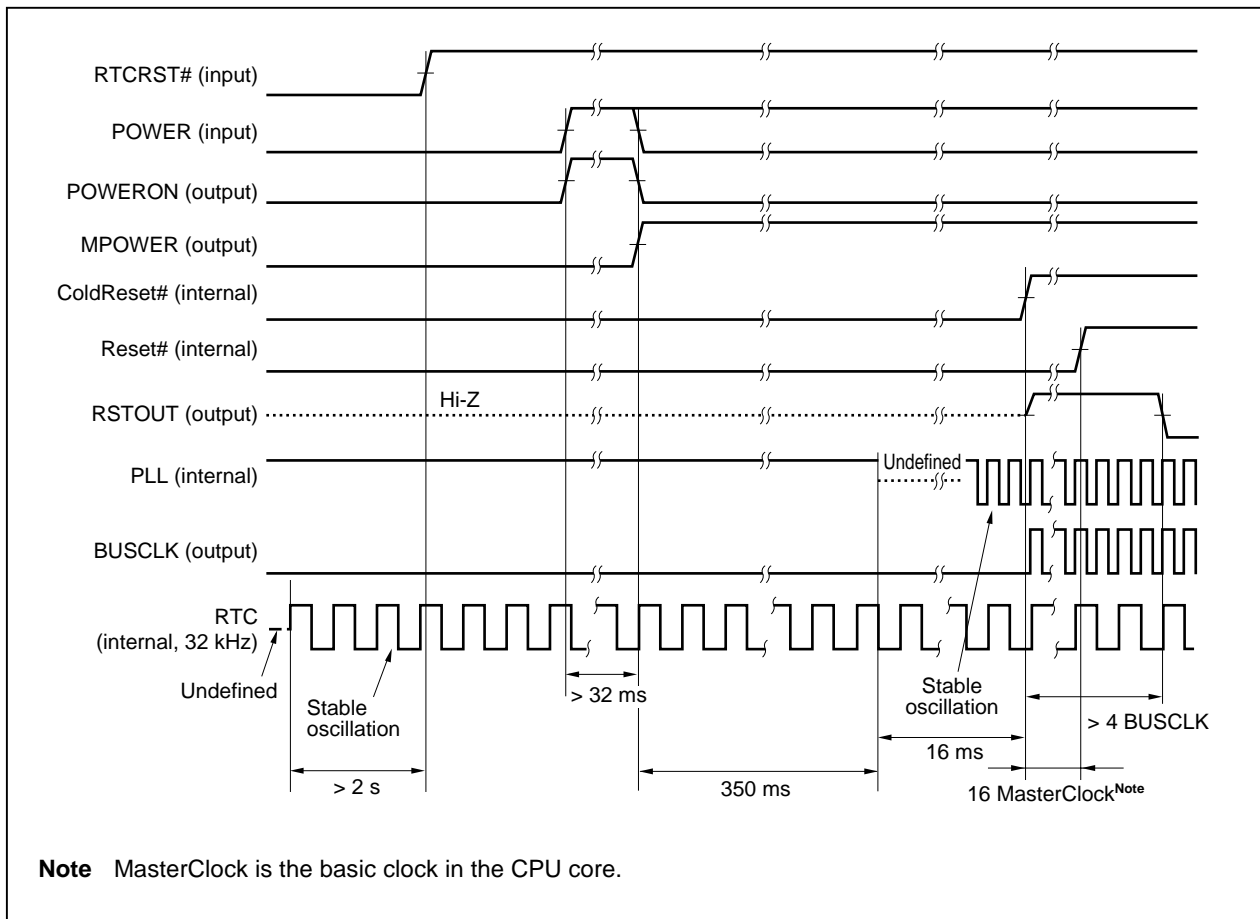
Figure 4-1. RTC Reset
