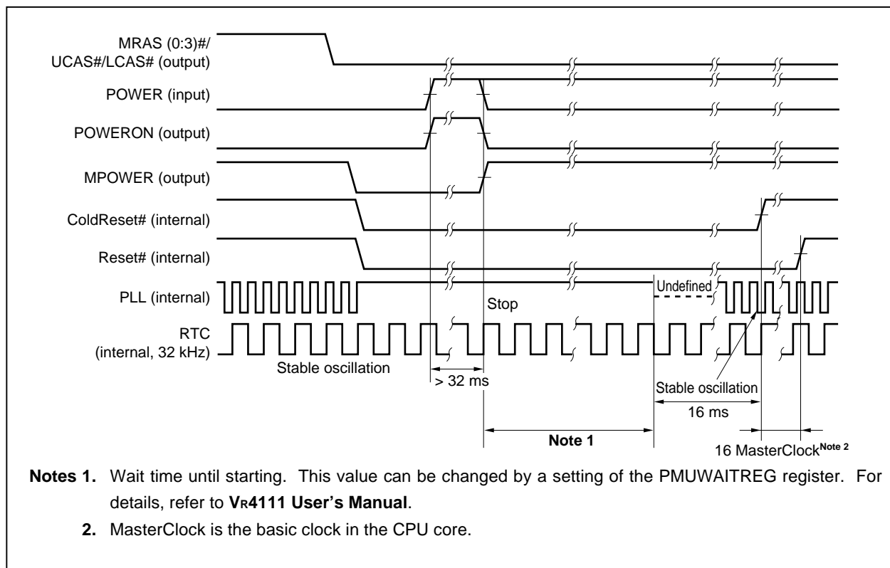
Figure 4-4. Software Shutdown
