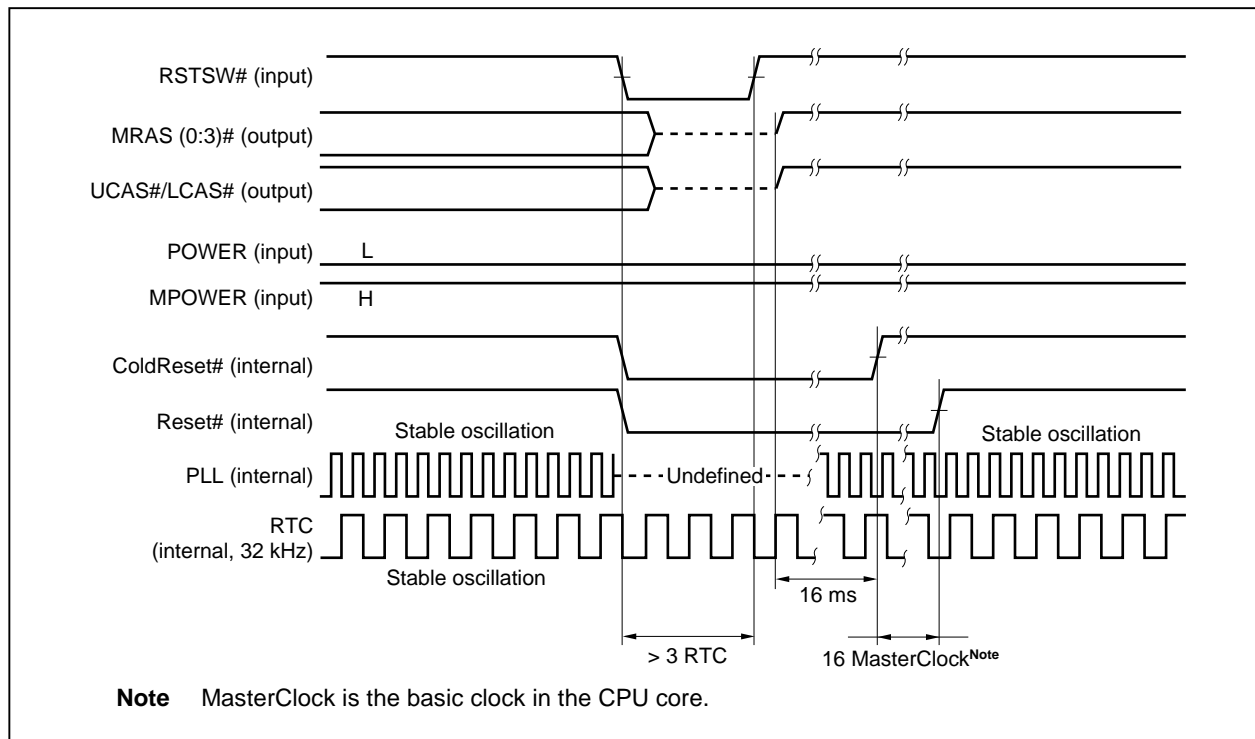
Figure 4-2. RSTSW
