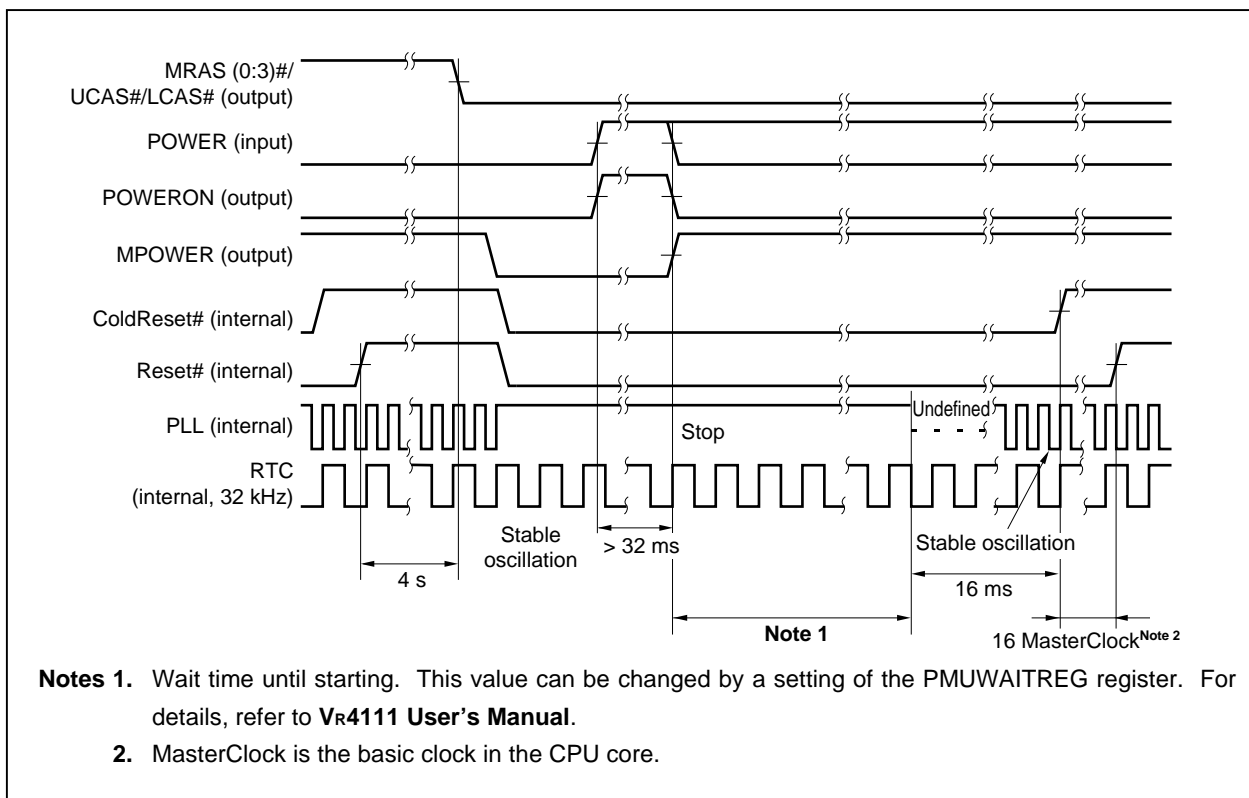
Figure 4-5. HALTimer Shutdown
