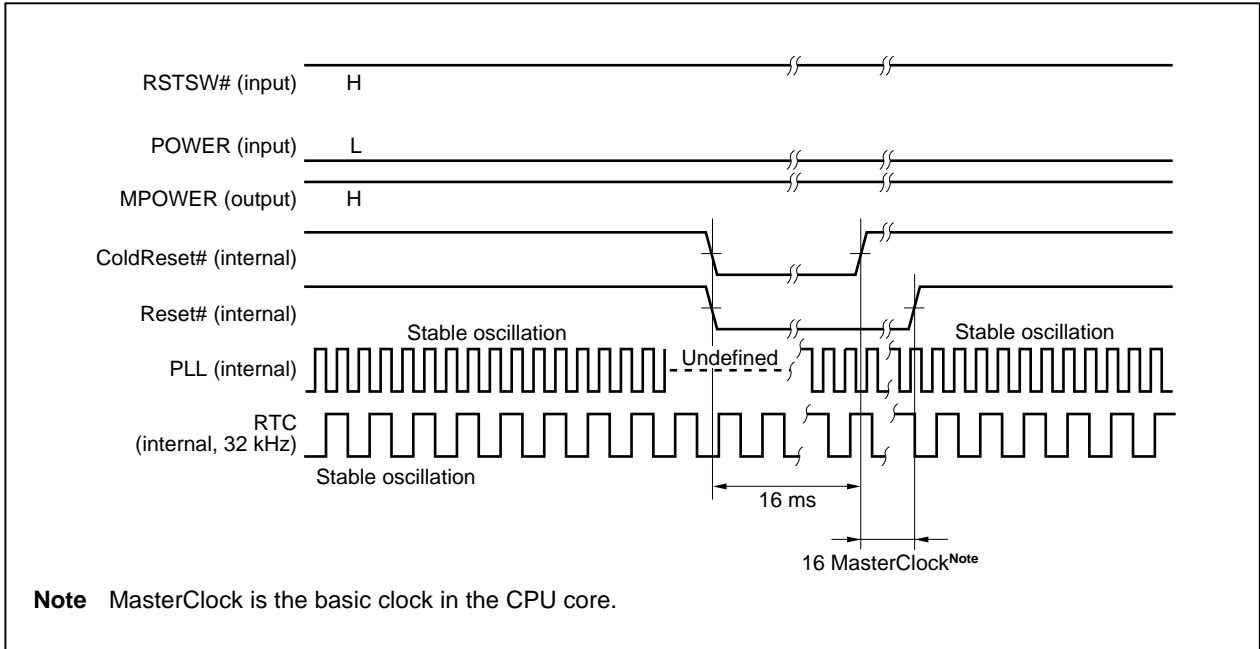
Figure 4-3. Deadman's SW
