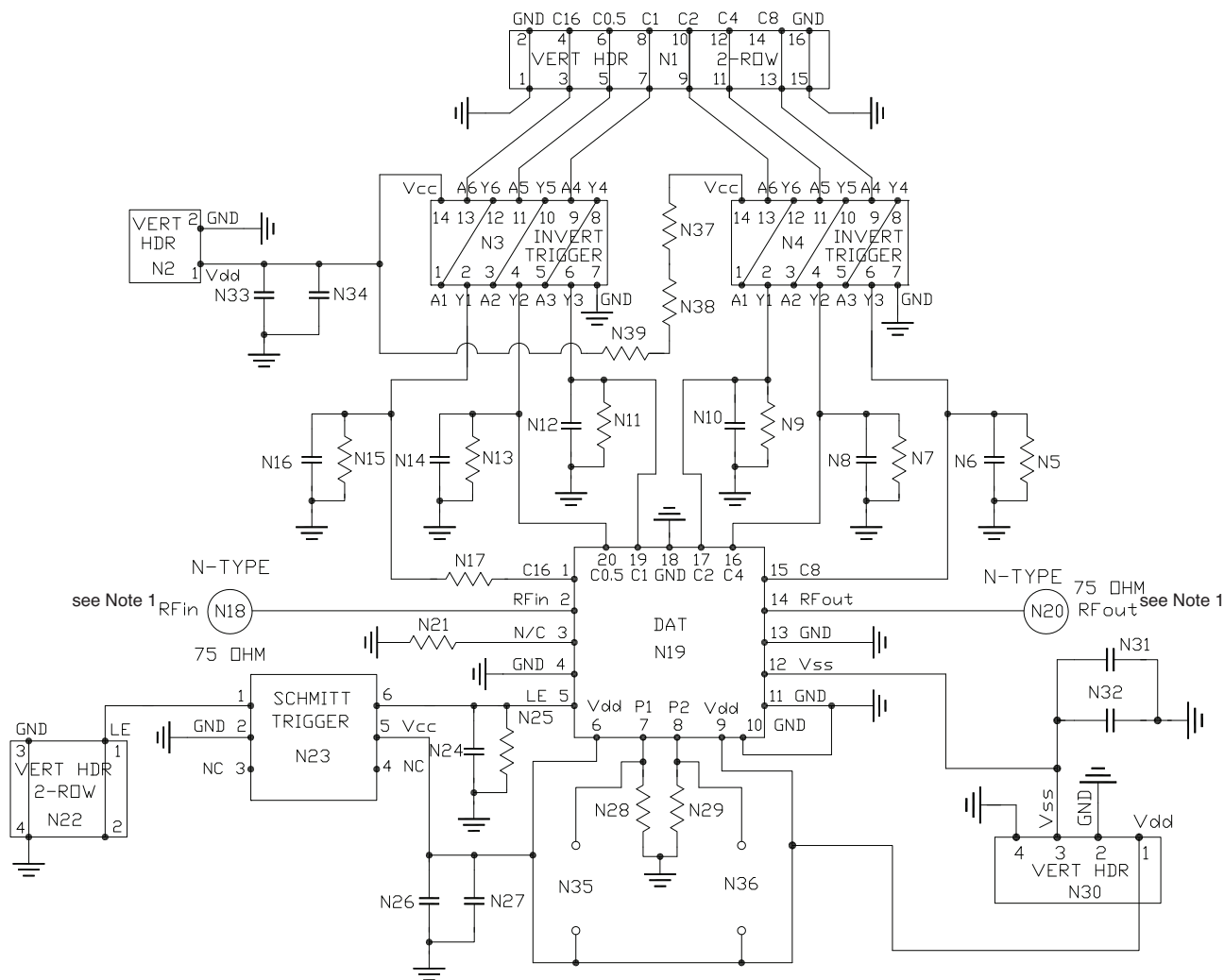
TB-341 Evaluation Board Schematic Diagram
