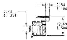
SECTION Y-Y
