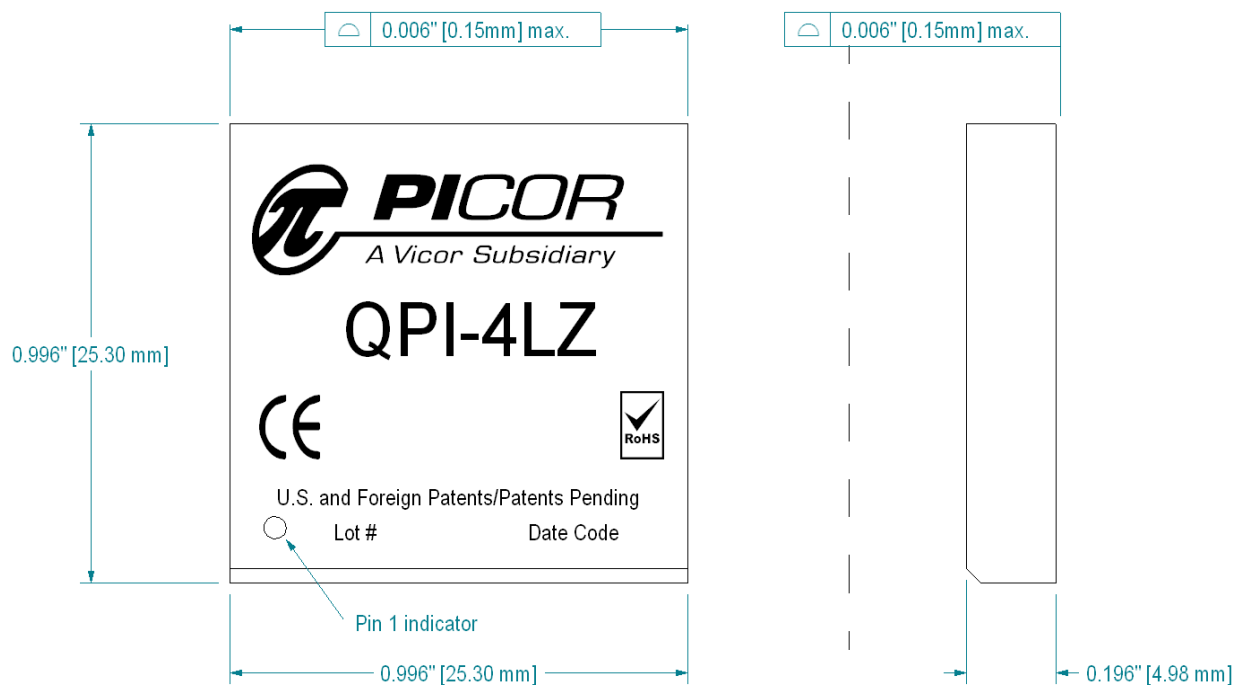
Figure 18 - Lidded Package Dimensions, tolerance of \pm 0.004 "
