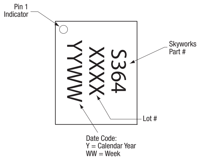
Figure 19. Typical Part Markings (Top View)
