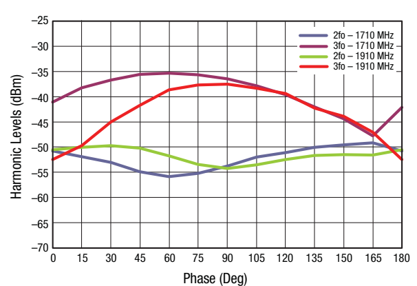
Figure 14. Harmonics vs Phase ( P_{IN} = +33 dBm, 5:1 VSWR Mismatch)
