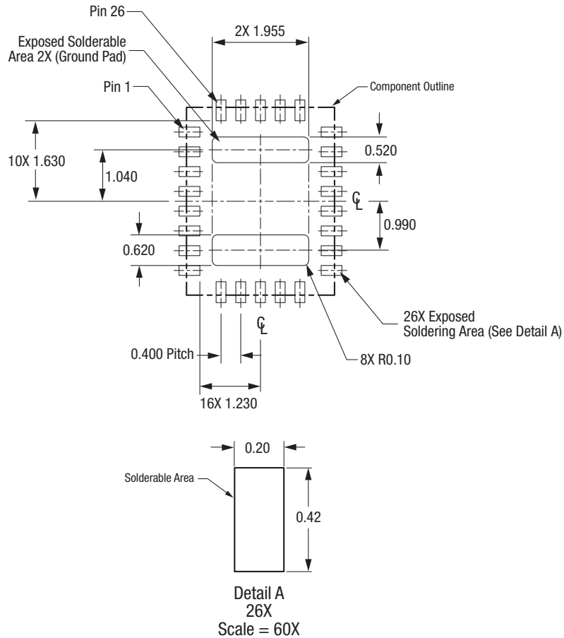
Figure 18. SKY13364-389LF PCB Layout Footprint (Top View)
