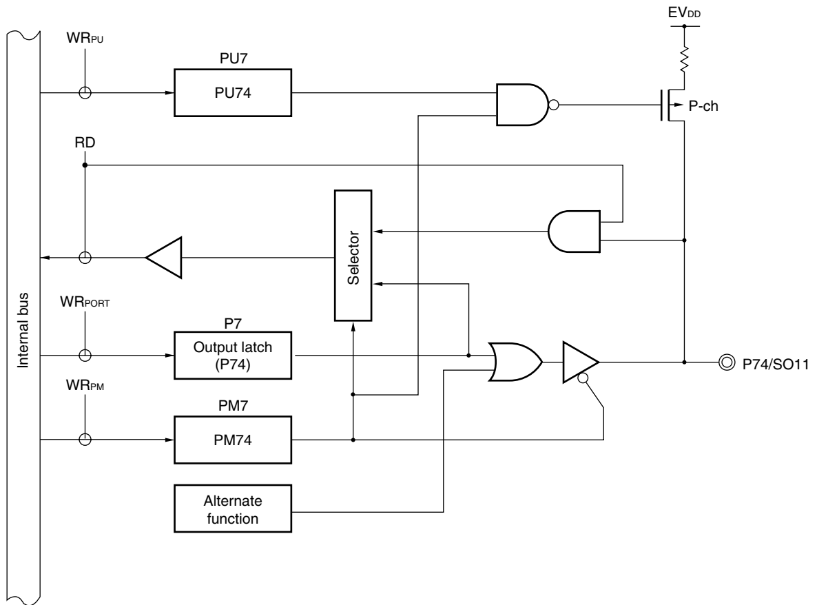
Figure 5-16. Block Diagram of P74
