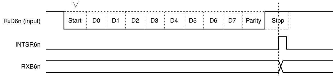
Figure 14-27. Reception Completion Interrupt Request Timing
