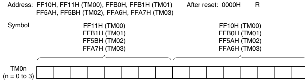
Figure 7-5. Format of 16-Bit Timer Counter 0n (TM0n)
