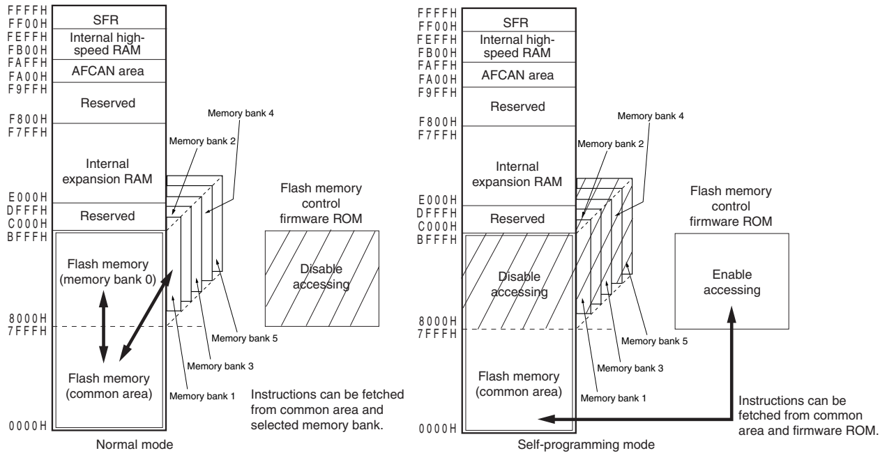
Figure 24-15. Operation Mode and Memory Map for Self-Programming (μPD78F0893)
