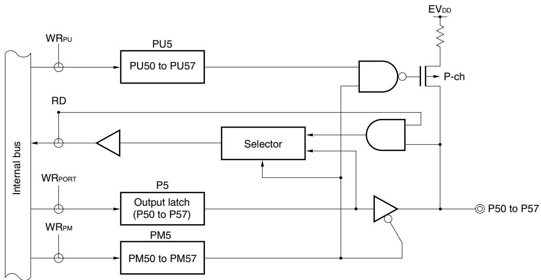
Figure 5-10. Block Diagram of P50 to P57
