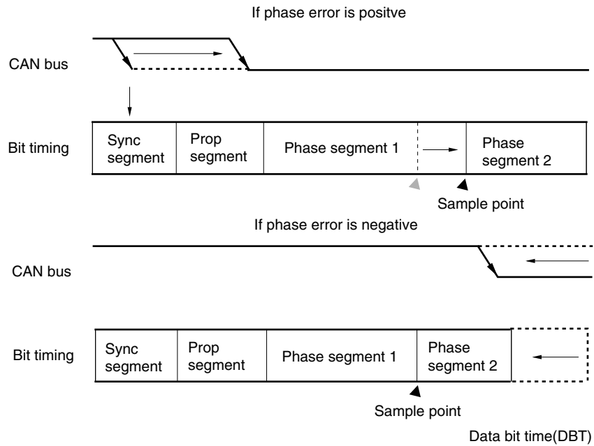
Figure 16-21. Resynchronization
