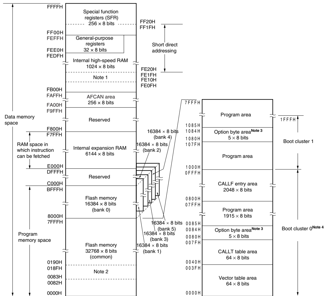
Figure 3-3. Memory Map (μPD78F0893)
