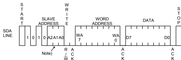
Fig.33 Byte write cycle (BR24S16-W)
