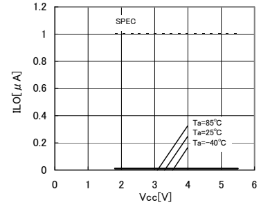
Fig.8 Output leak current I_{LO}(\text{SDA})
