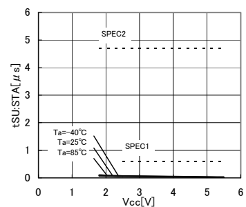
Fig.20 Start condition setup time t_{SU:STA}
