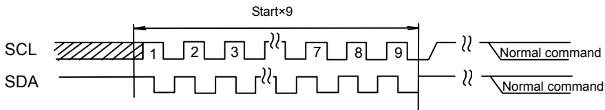
Fig.48-(c) START x 9+ command input
