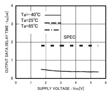
Fig.23 'H' Data output delay time t_{PD1}
