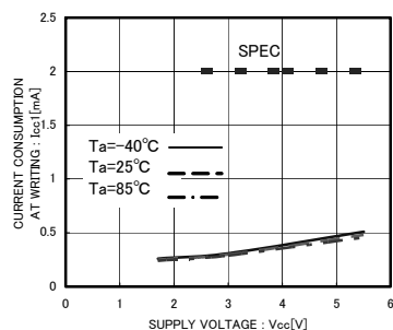
Fig.9 Current consumption at WRITE operation I_{CC1} ( f_{SCL}=400\text{kHz} BR24S16/32/64-W)
