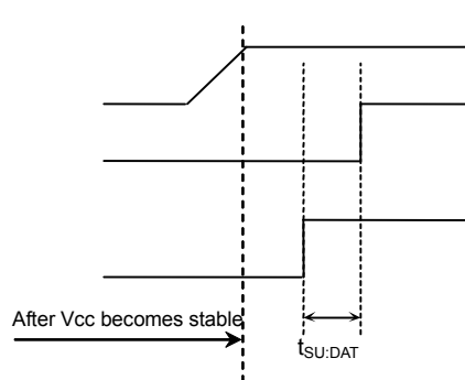
Fig.62 When SCL='L' and SDA='L'
