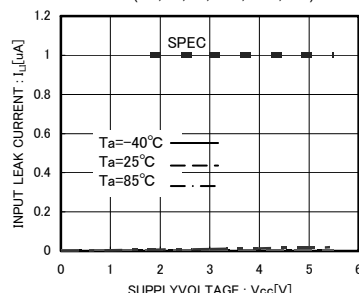
Fig.7 Input leak current I_L (A0,A1,A2,SCL,WP)
