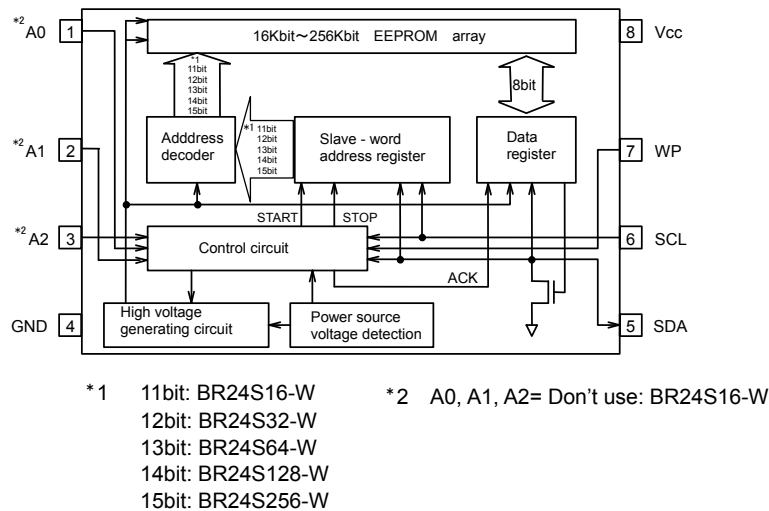
Fig.2 Block diagram
