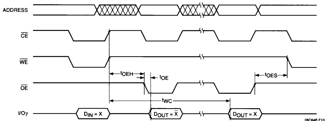
Figure 7. DATA Polling
