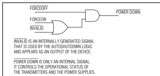
Figure 3c. MAX32xxE AutoShutdown Logic
