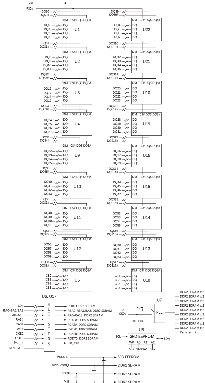
Figure 2: Functional Block Diagram
