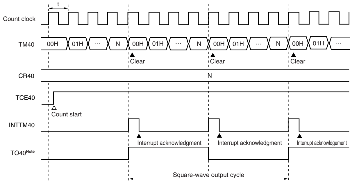
Figure 6-14. Timing of Square-Wave Output with 8-Bit Resolution
