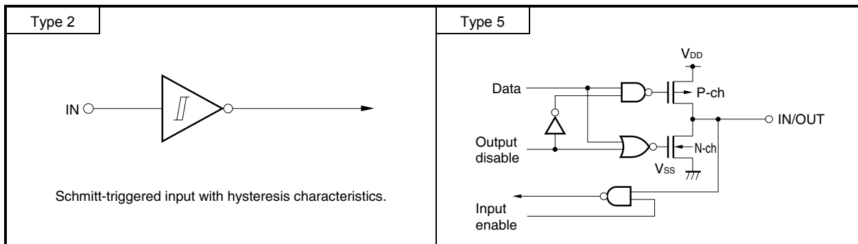
Figure 2-1. I/O Circuit Type (1/2)
