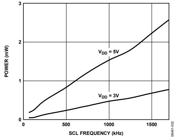
Figure 17. Power vs. SCL Frequency, V_{REF} = 2.5\text{ V}
