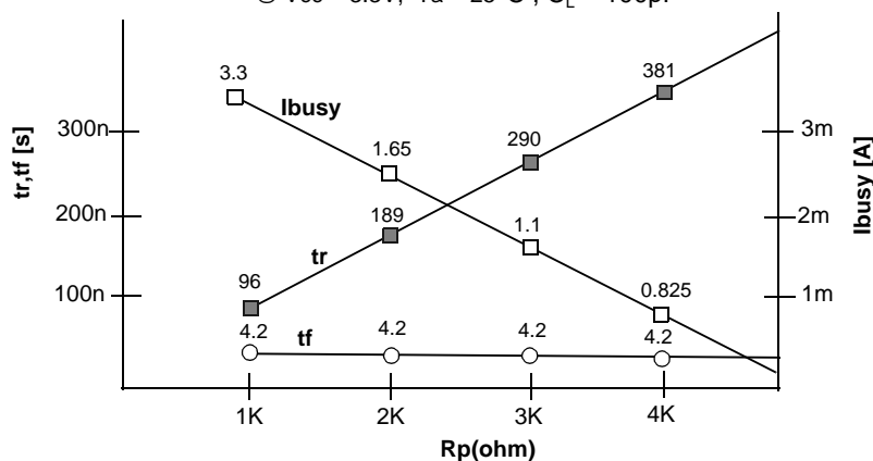
Figure 17 Rp vs tr,tf & Rp vs i_{\text{busy}}
