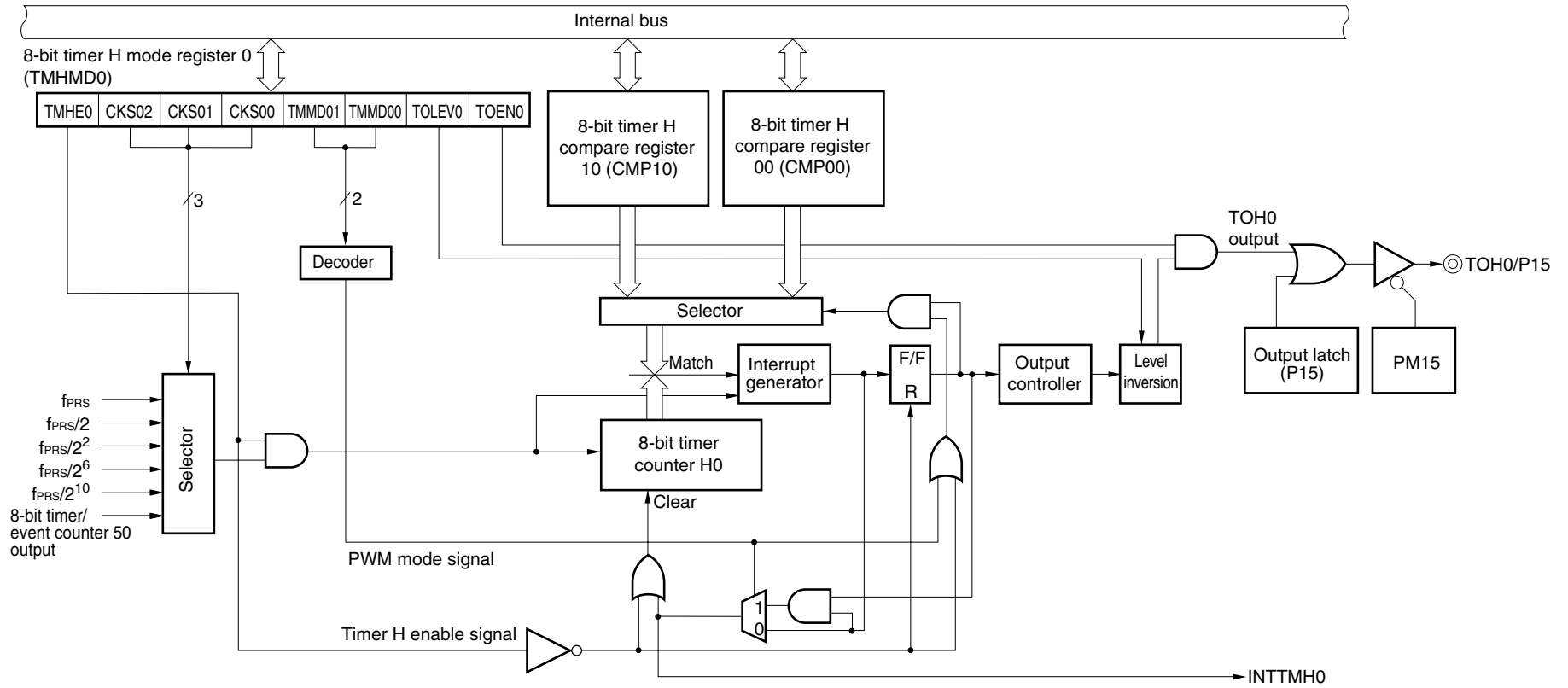
&lt;R&gt; Figure 8-1. Block Diagram of 8-bit Timer H0
