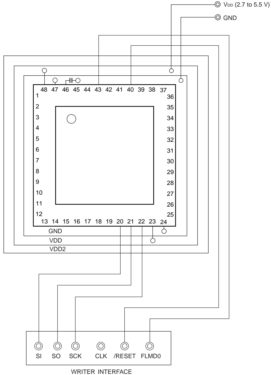
Figure 25-7. Example of Wiring Adapter for Flash Memory Writing in 3-Wire Serial I/O (CS110) Mode (48-Pin Products)
