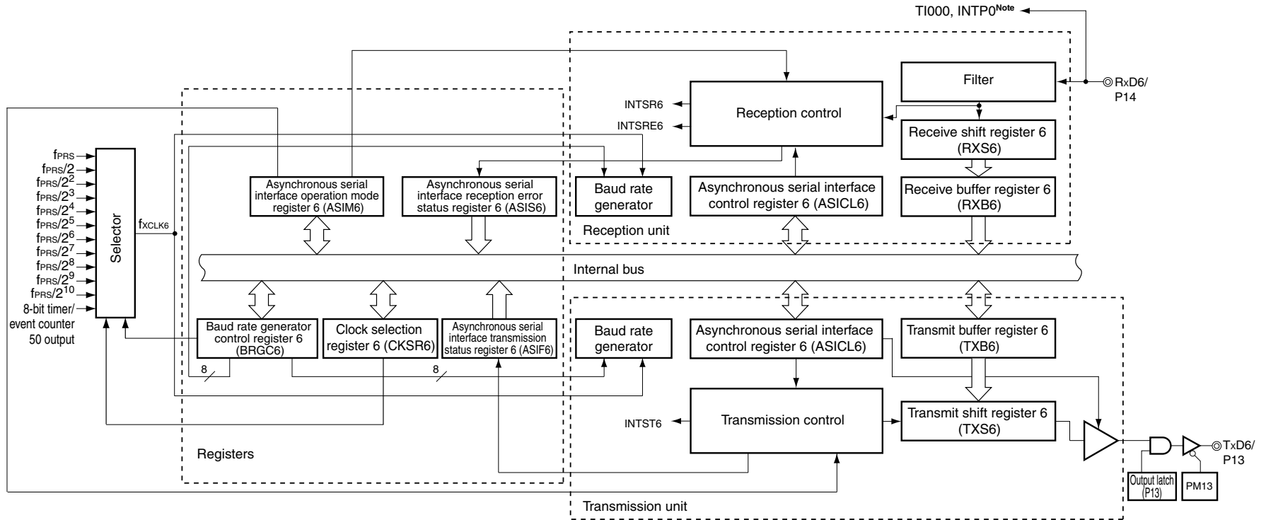
&lt;R&gt;Figure 14-4. Block Diagram of Serial Interface UART6
