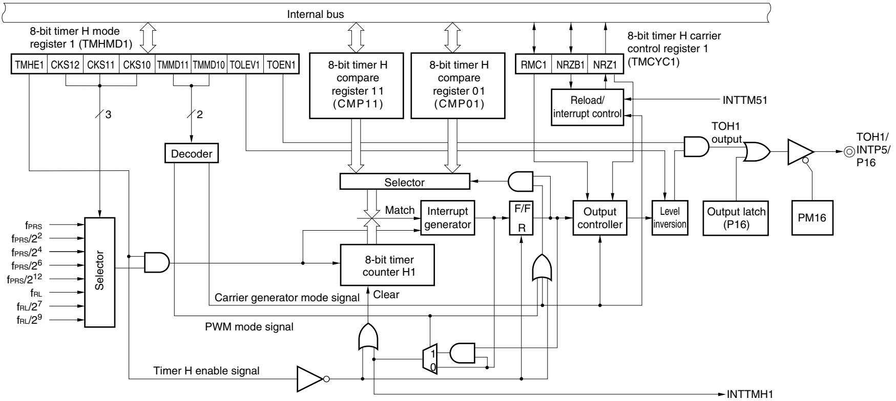
&lt;R&gt; Figure 8-2. Block Diagram of 8-bit Timer H1
