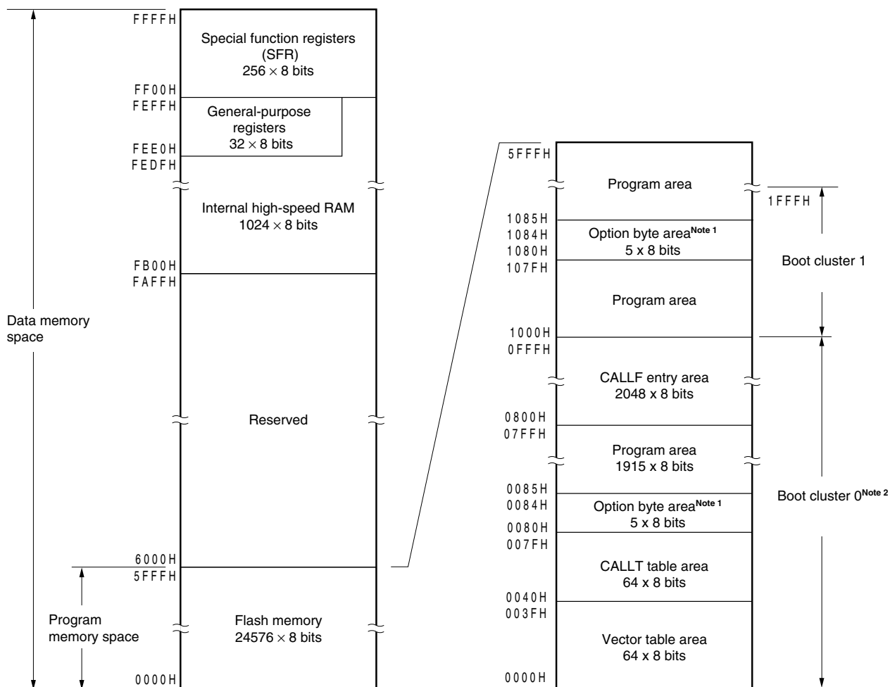
Figure 3-2. Memory Map ( \mu PD78F0512)
