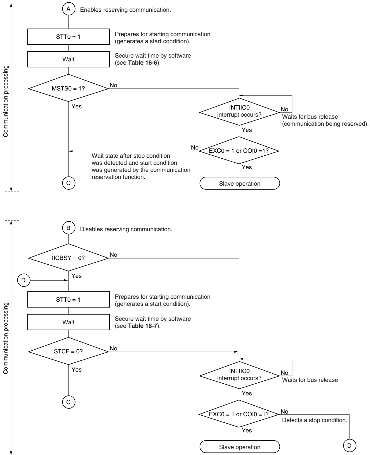
Figure 16-24. Master Operation in Multi-Master System (2/3)
