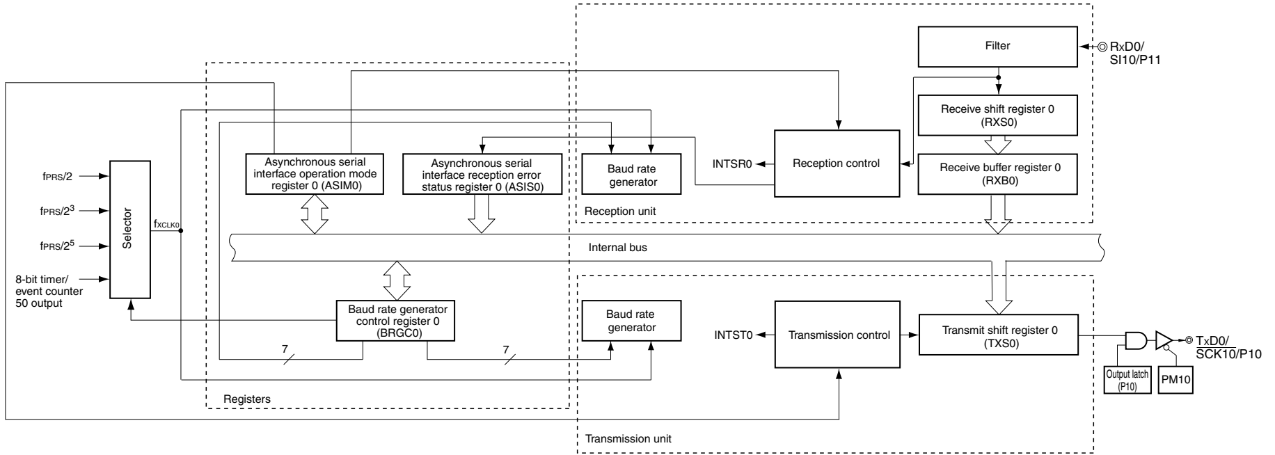
&lt;R&gt; Figure 13-1. Block Diagram of Serial Interface UART0
