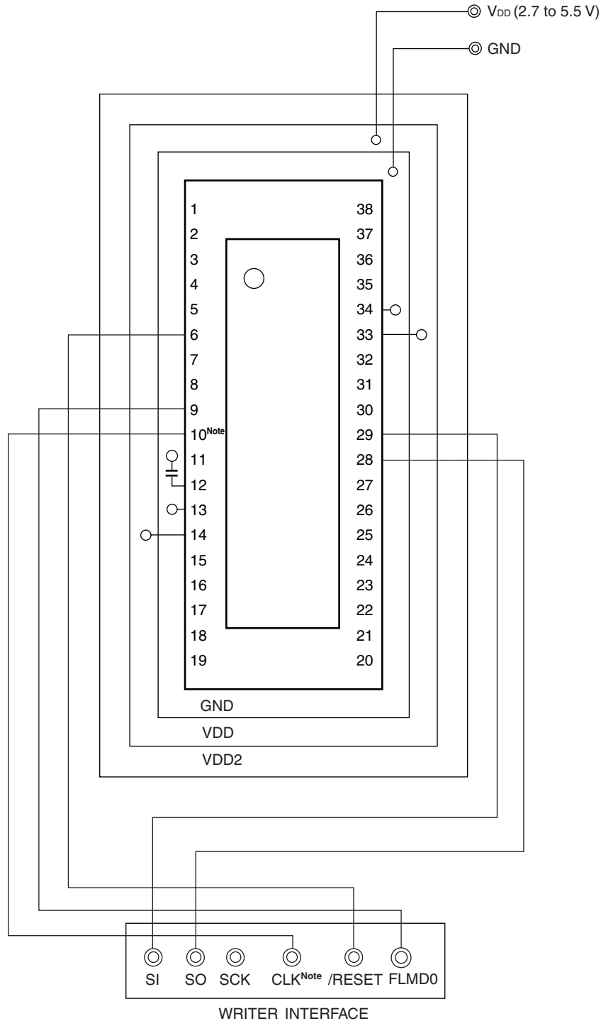
Figure 25-4. Example of Wiring Adapter for Flash Memory Writing in UART (UART6) Mode (38-Pin Products)
