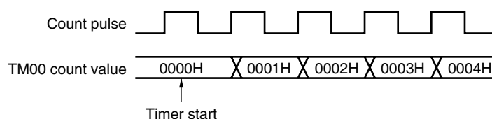
Figure 6-55. Start Timing of TM00 Count
