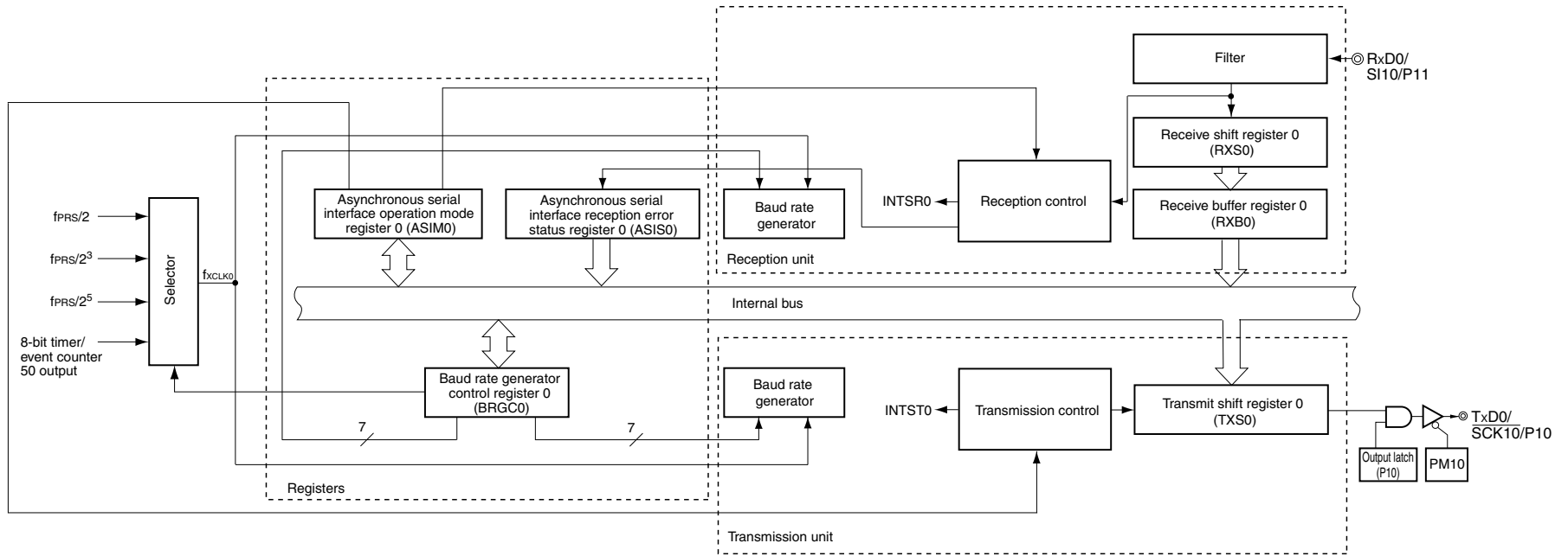
&lt;R&gt; Figure 14-1. Block Diagram of Serial Interface UART0
