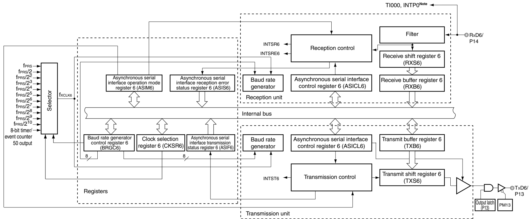
&lt;R&gt; Figure 15-4. Block Diagram of Serial Interface UART6
