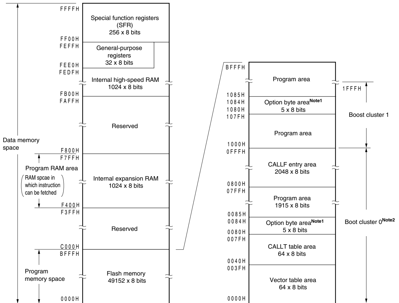
Figure 3-4. Memory Map (μPD78F0534)
