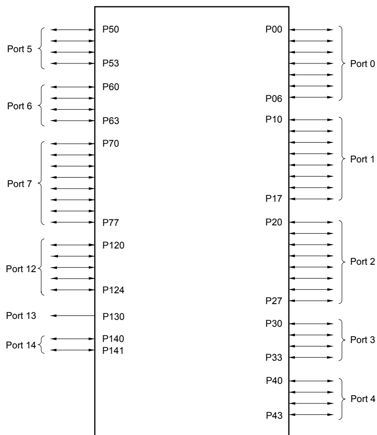
Figure 5-1. Port Types
