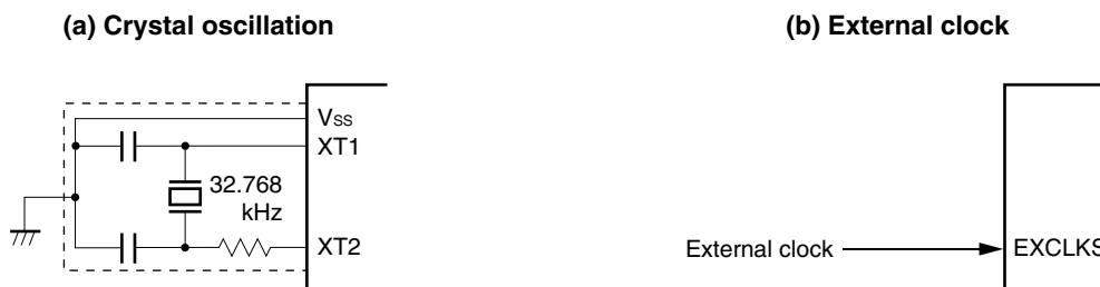
Figure 6-10. Example of External Circuit of XT1 Oscillator
