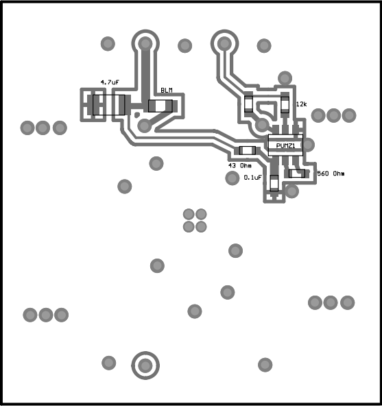
Evaluation Board Layout (Bottom View)
