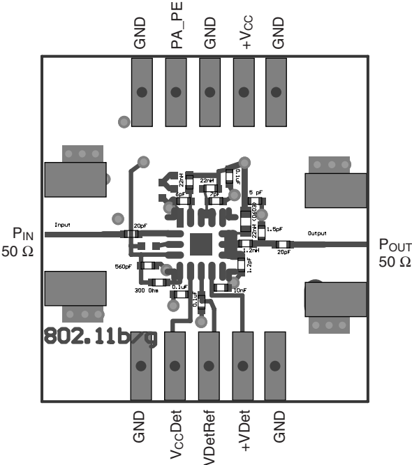
Evaluation Board Layout (Top View)
