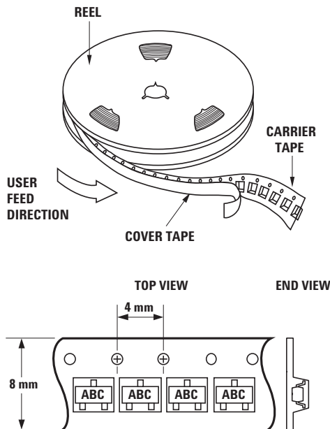
Figure 4. Option -TR1/-TR2 for SOT-23 Packages.
