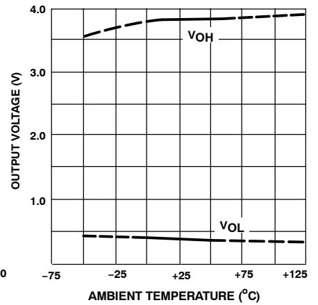
Figure 8. Output Voltage vs. Ambient Temperature
