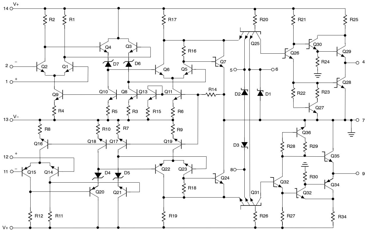
Figure 2. Equivalent Schematic
