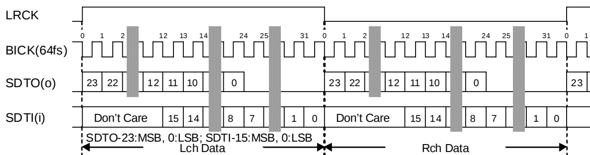
Figure 3. PORT1= Mode0/2, PORT2=Mode0 Timing
