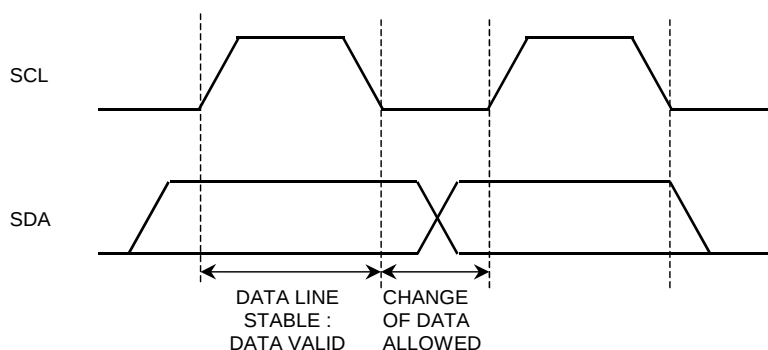
Figure 11. Data Transfer
