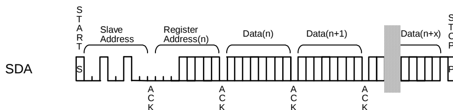
Figure 17. WRITE Operation
