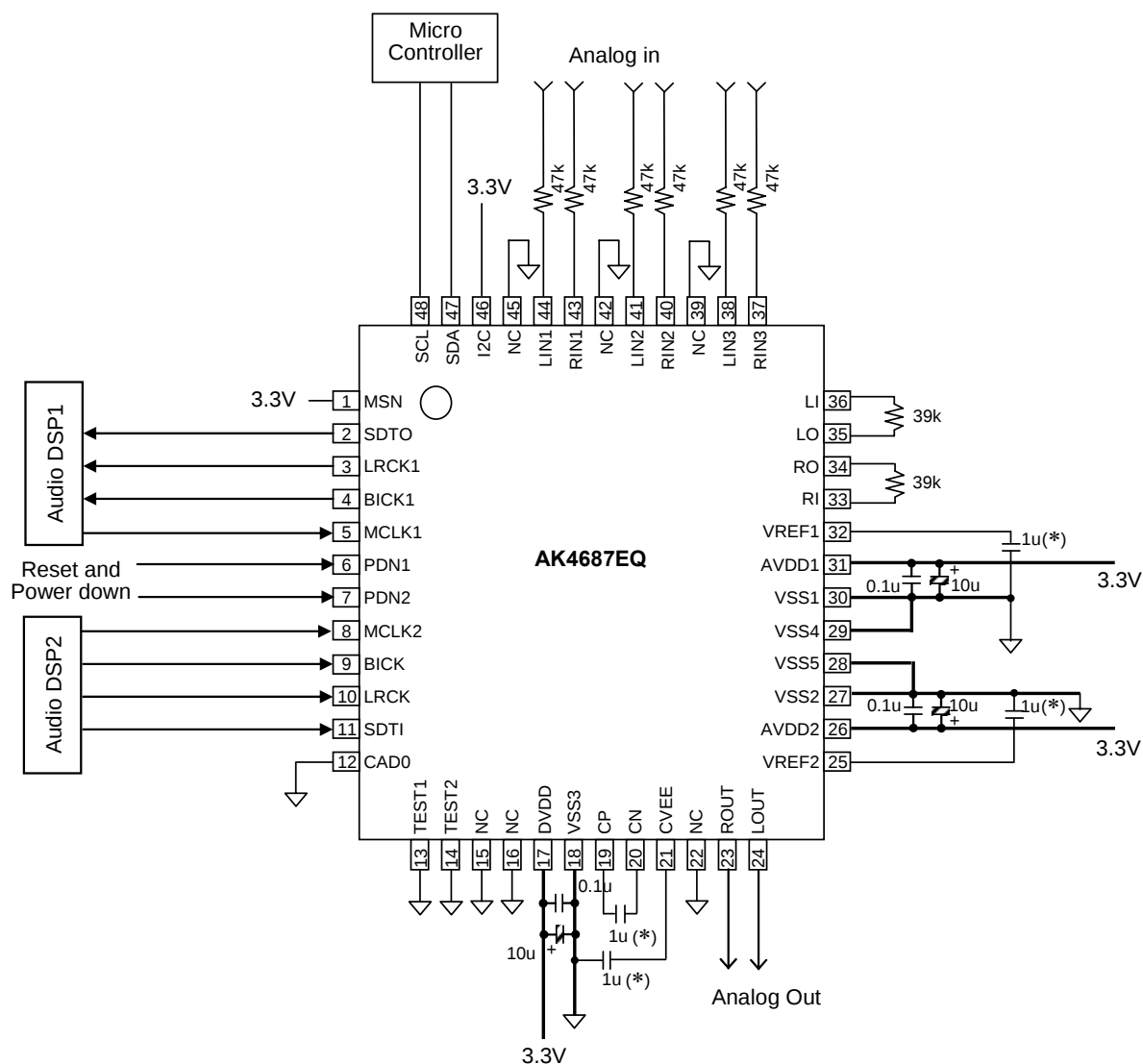
Figure 20. Typical Connection Diagram (I 2 C Control mode, CAD0 pin = “L”, Master mode)
