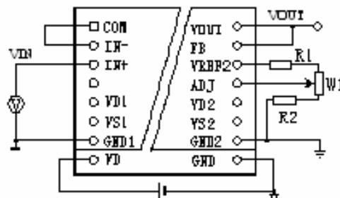
Wiring Diagram
