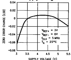
Zero Error Change vs Supply Voltage
