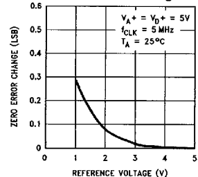
Zero Error Change vs Reference Voltage
