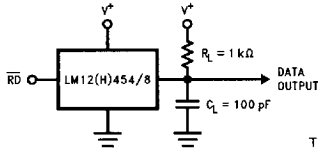
FIGURE 7. TRI-STATE Test Circuits and Waveforms
