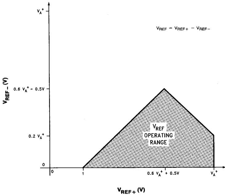
FIGURE 3. The General Case of the V_{REF} Operating Range
