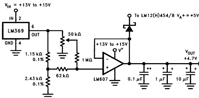
FIGURE 12. Low Drift Extremely Stable Reference Circuit
