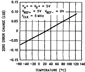
Zero Error Change vs Temperature
