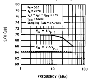
Unipolar Signal-to-Noise Ratio vs Input Frequency
