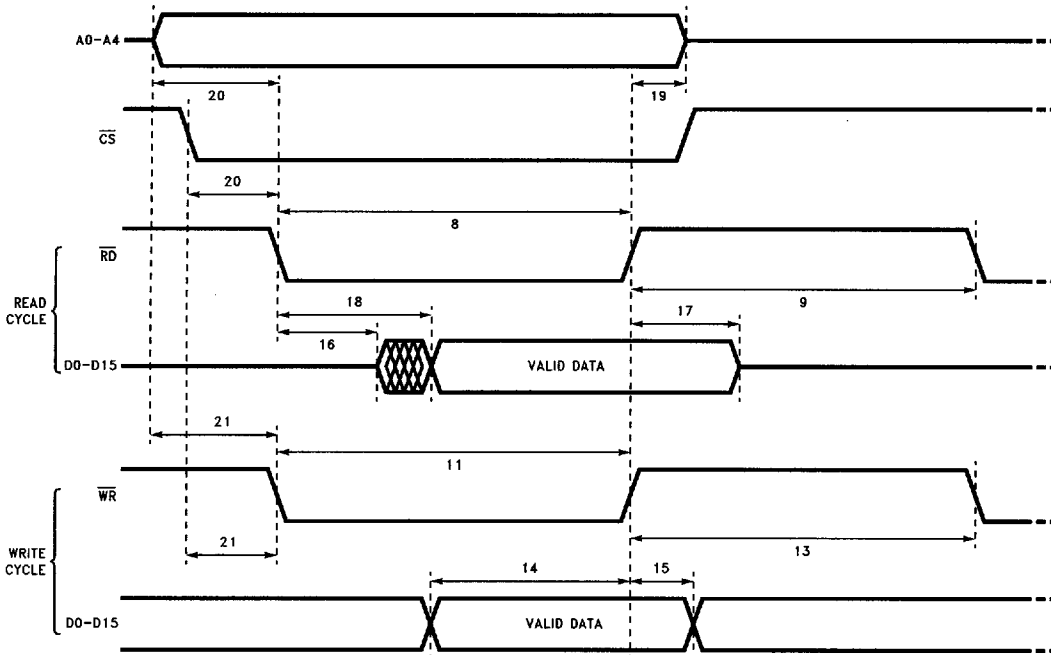
FIGURE 8b. Non-Multiplexed Data Bus (ALE = 1)
