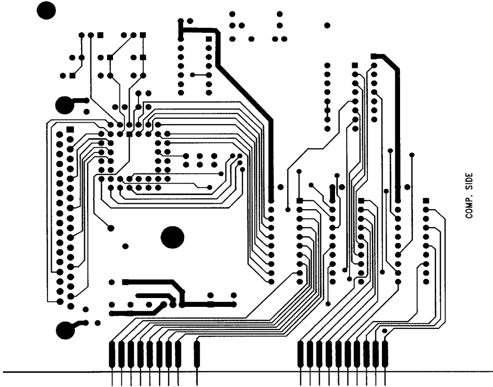
FIGURE 17. LM12(H)454/8 Evaluation/Interface Board Component-Side Layout Positive
