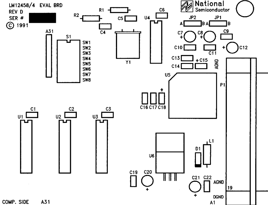
FIGURE 16. Silk-Screen Layout Showing Parts Placement on the LM12(H)454/8 Evaluation/Interface Board
