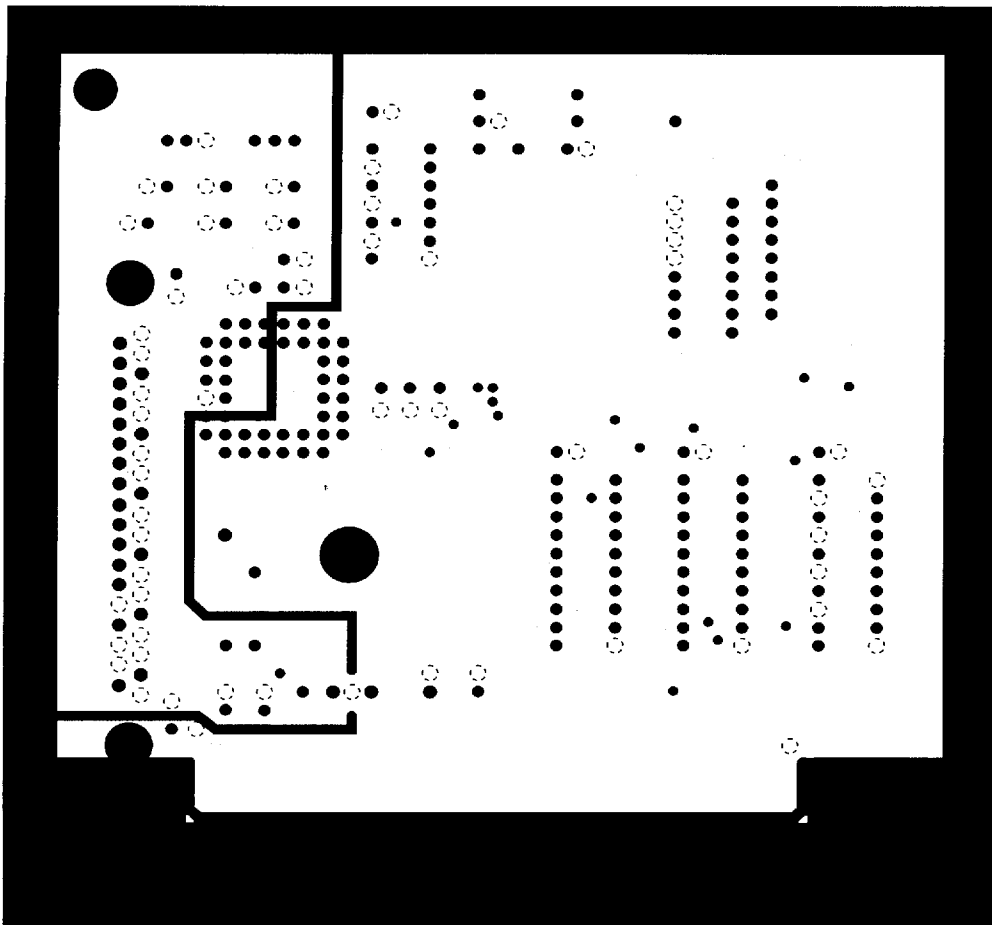
FIGURE 18. LM12(H)454/8 Evaluation/Interface Board Ground-Plane Layout Negative
