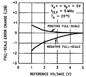
Full-Scale Error Change vs Reference Voltage
