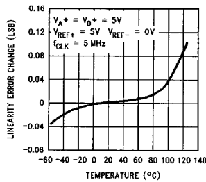
Linearity Error Change vs Temperature
