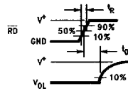
FIGURE 7. TRI-STATE Test Circuits and Waveforms
