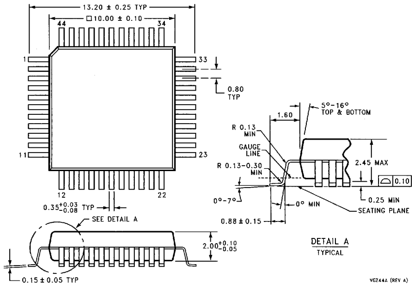
Order Number LM12H458CIVF or LM12458CIVF NS Package Number VG244A
