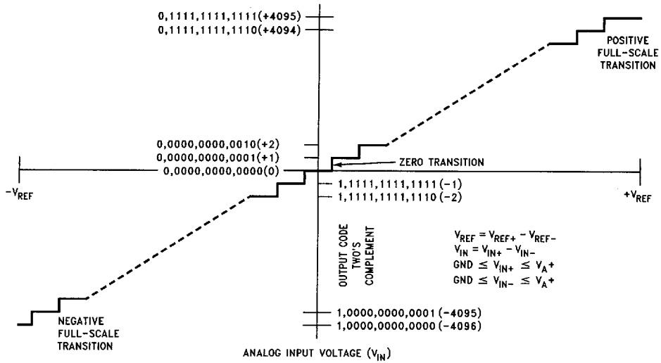
FIGURE 5a. Transfer Characteristic
