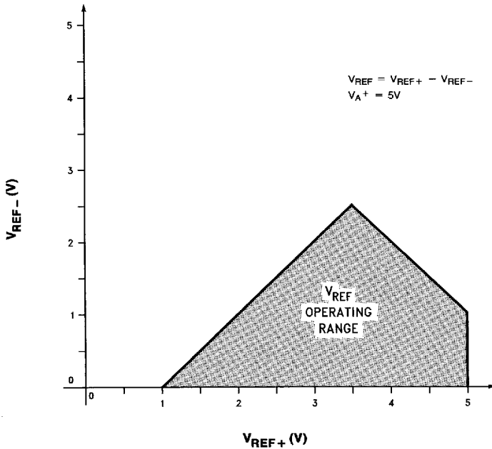
FIGURE 4. The Specific Case of the V_{REF} Operating Range for V_A^+ = 5V
