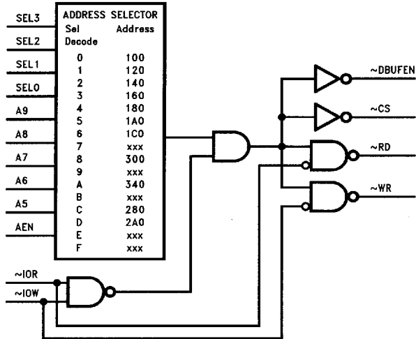
FIGURE 15. GAL Functional Block Diagram
