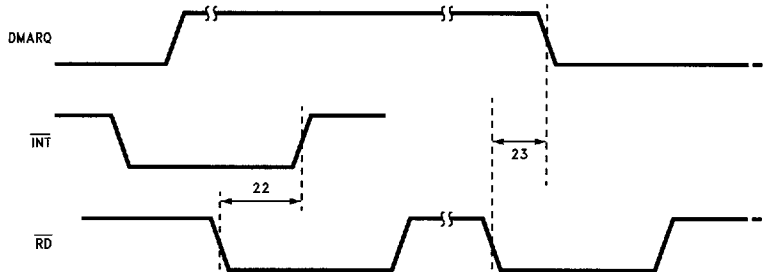
FIGURE 8c. Interrupt and DMARQ
