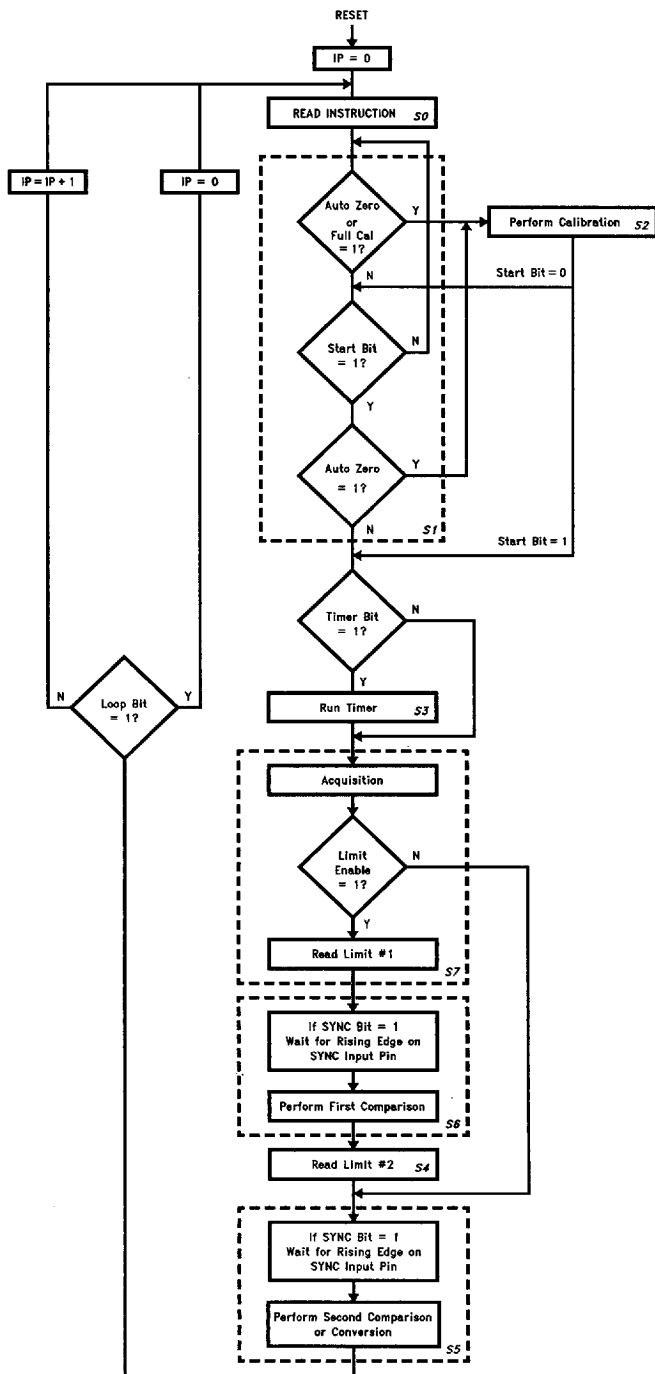
FIGURE 11. Sequencer Logic Flow Chart (IP = Instruction Pointer)
