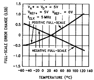
Full-Scale Error Change vs Temperature
