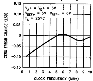
Zero Error Change vs Clock Frequency
