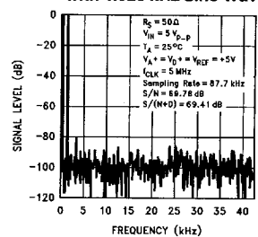
Unipolar Spectral Response with 1.028 kHz Sine Wave Input
