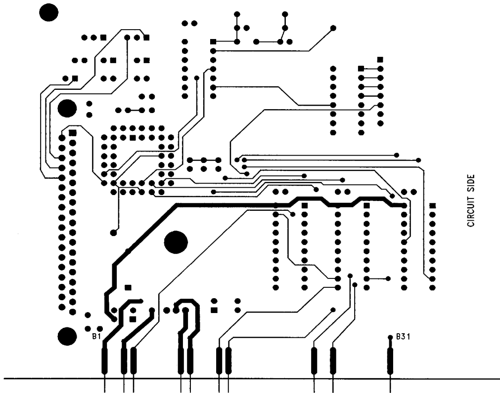
FIGURE 19. LM12(H)454/8 Evaluation/Interface Circuit-Side Layout Positive
