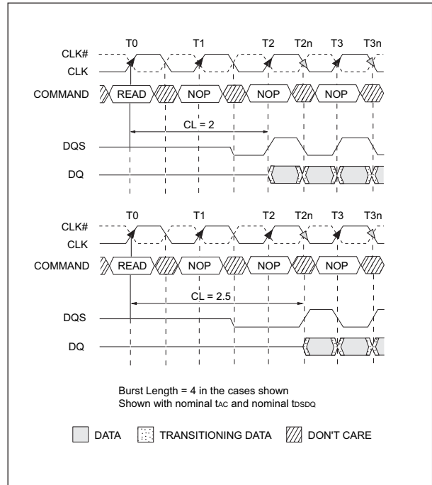
FIGURE 4 – CAS LATENCY
