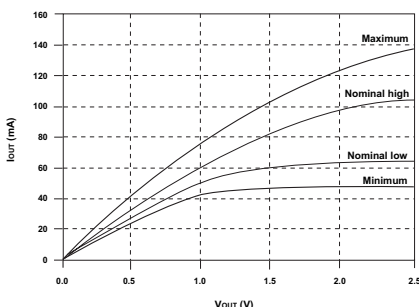
FIGURE A FULL DRIVE PULL-DOWN CHARACTERISTICS
