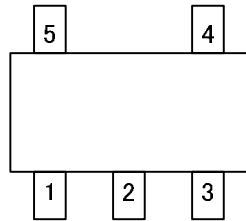
SOT-25(TOP VIEW)
