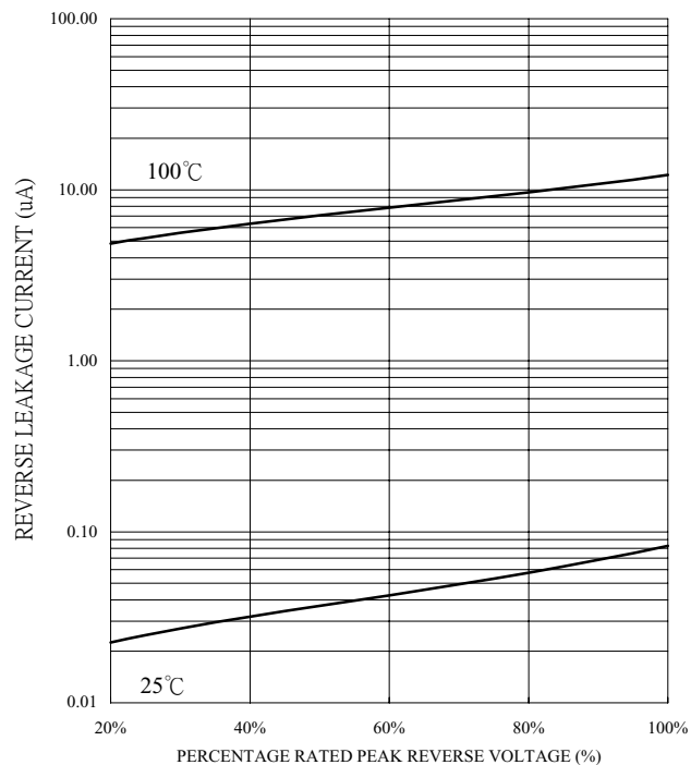
FIG. 5-TYPICAL REVERSE CHARACTERISTICS
