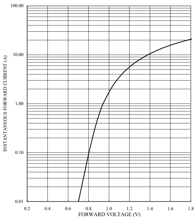
FIG. 2-TYPICAL FORWARD CHARACTERISTICS
