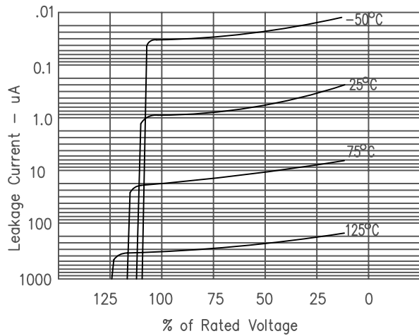
Figure 2 Typical Reverse Leakage Current
