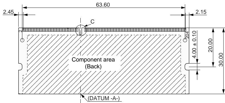
Detail A
