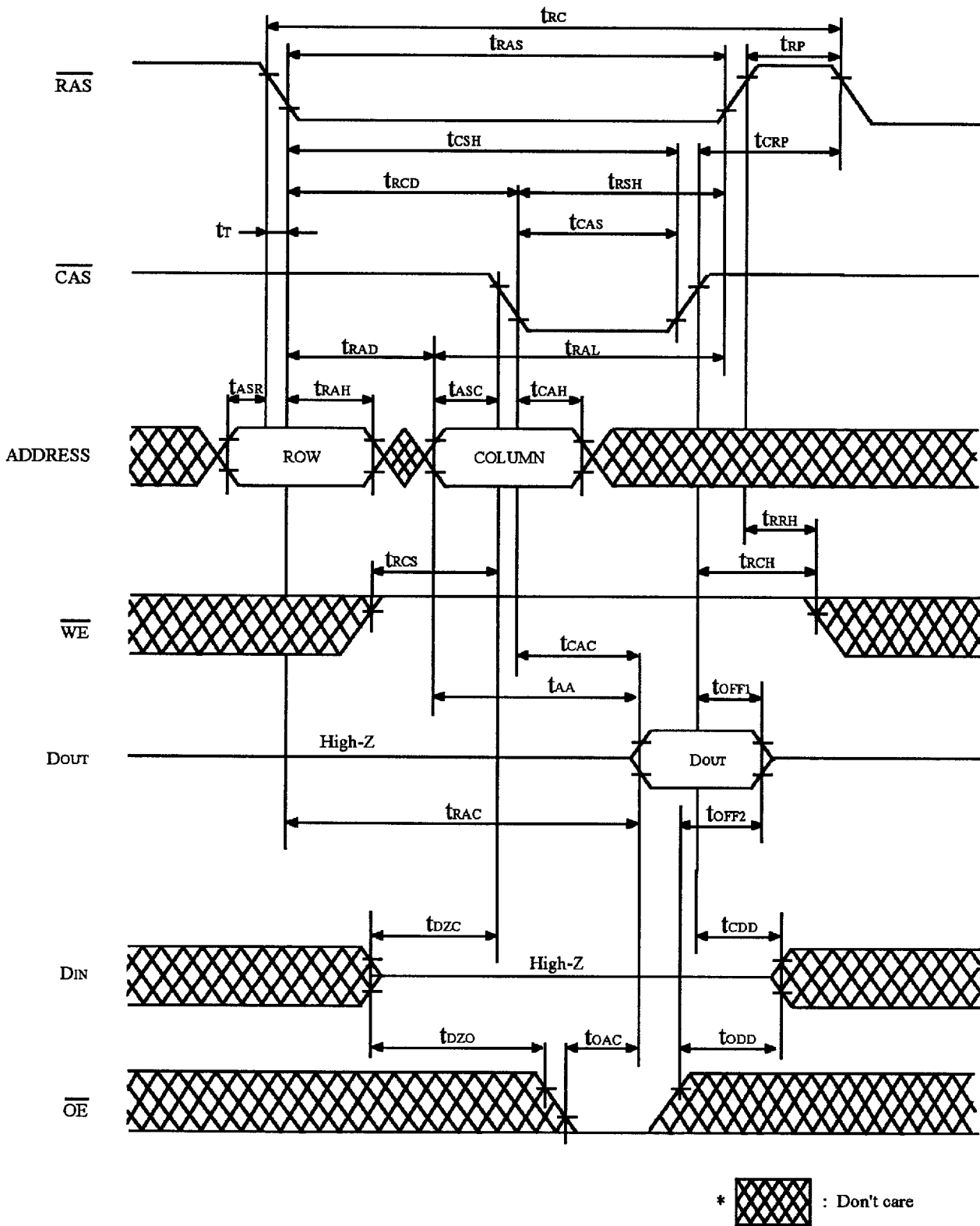
FIGURE 1. READ CYCLE
