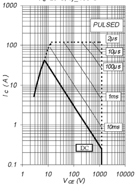
Fig.3 - Forward SOA T_c=25^{\circ}C ; T_j \leq 150^{\circ}C
