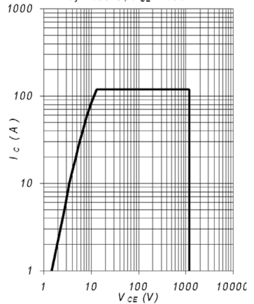
Fig.4 - Reverse Bias SOA T_j = 150^{\circ}C , V_{GE} = 15V
