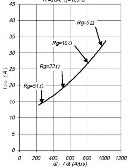
Fig.19 - Typical Diode I_{RR} vs di_F/dt V_{CC}=600\text{V}; V_{CE}=15\text{V} I_F=20\text{A}; T_j=125^\circ\text{C}
