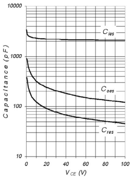
Fig.22 - Typical Capacitance vs V_{CE} V_{GE}=0V ; f=1MHz
