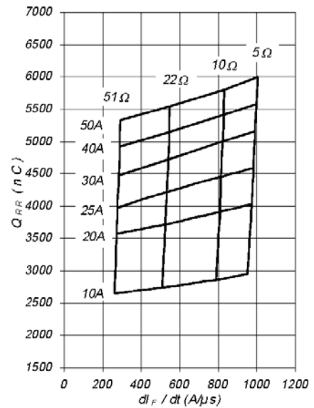
Fig.20 - Typical Diode Q_{RR} V_{CC}=600\text{V}; V_{CE}=15\text{V}; T_j=125^\circ\text{C}
