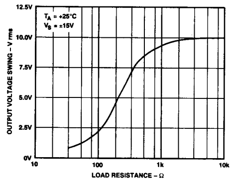
Figure 14. Output Voltage Swing vs. Load Resistance
