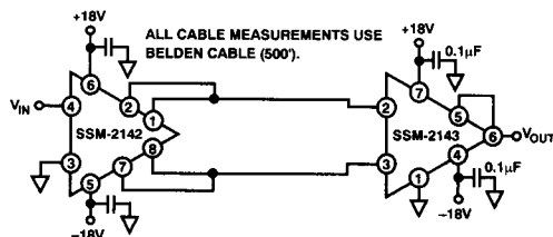
Figure 29. SSM-2142/SSM-2143 Balanced Line Driver/Receiver System
