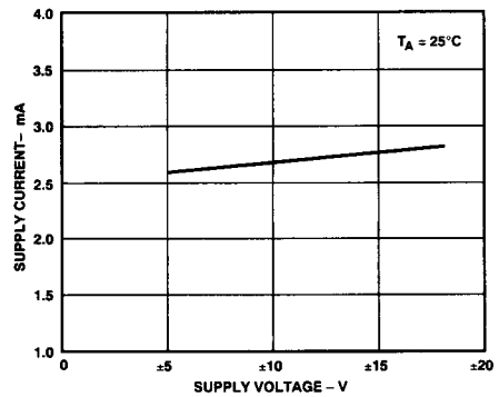
Figure 24. Supply Current vs. Supply Voltage
