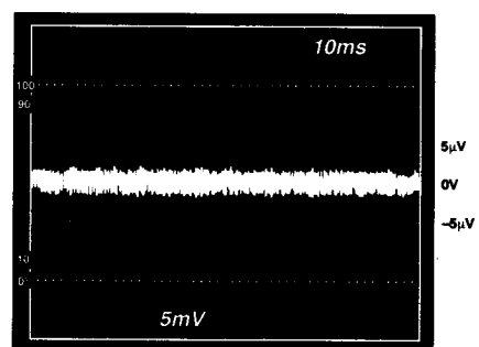
Figure 18. Voltage Noise from 0 kHz to 1 kHz*
