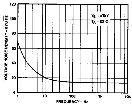
Figure 16. Voltage Noise Density vs. Frequency
