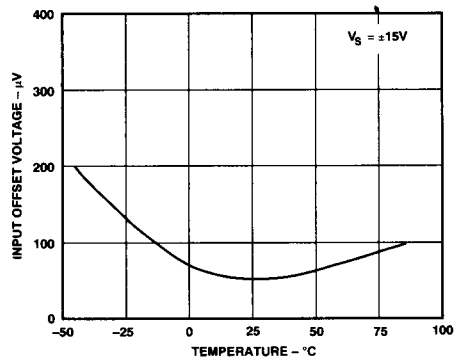
Figure 22. Input Offset Voltage vs. Temperature
