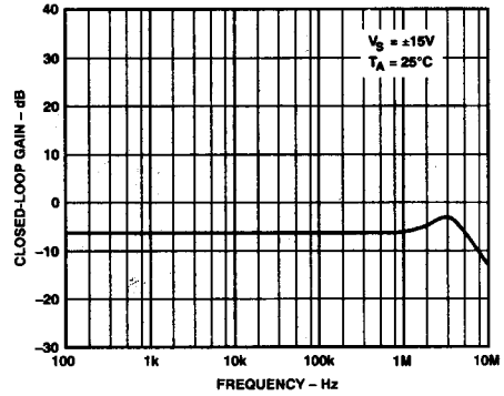
Figure 8. Closed-Loop Gain vs. Frequency, 100 Hz to 10 MHz
