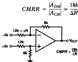
Figure 27. A Small Mismatch in Resistance Results in a Large Common-Mode Error.
