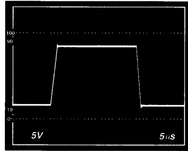
Figure 2. Large Signal Transient Response ( V_{IN} = +24\text{dBu} , G = 1/2 , R_L = 2\text{k}\Omega , V_S = \pm 15\text{V} , T_A = +25^\circ\text{C} )
