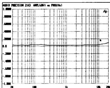
Figure 33. SSM-2142/SSM-2143 System Frequency Response ( V_S = \pm 18 V , V_{IN} = 0 dBV, 500' Cable)
