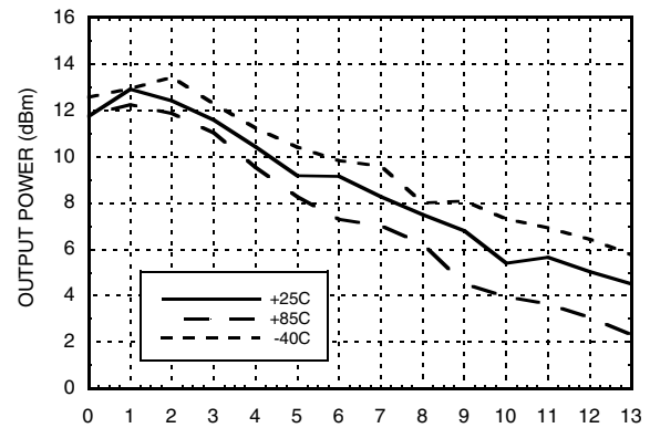
Output Power vs. Tuning Voltage, Vcc = +5V
