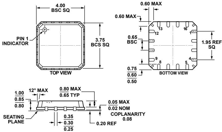
Figure 73. 16-Lead Lead Frame Chip Scale Package [LFCSQ_VQ] 4 mm × 4 mm Body, Very Thin Quad, with Hidden Paddle (CP-16-19)
