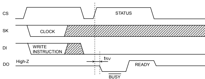
Fig.48 \overline{R/B} status output timing chart
