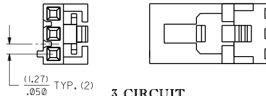
3 CIRCUIT
