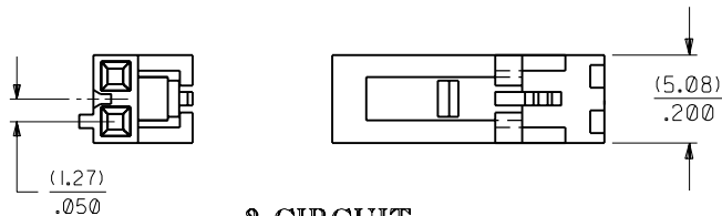
2 CIRCUIT
