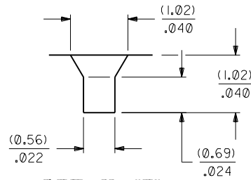
DETAIL "F" TYP. SCALE 20:1
