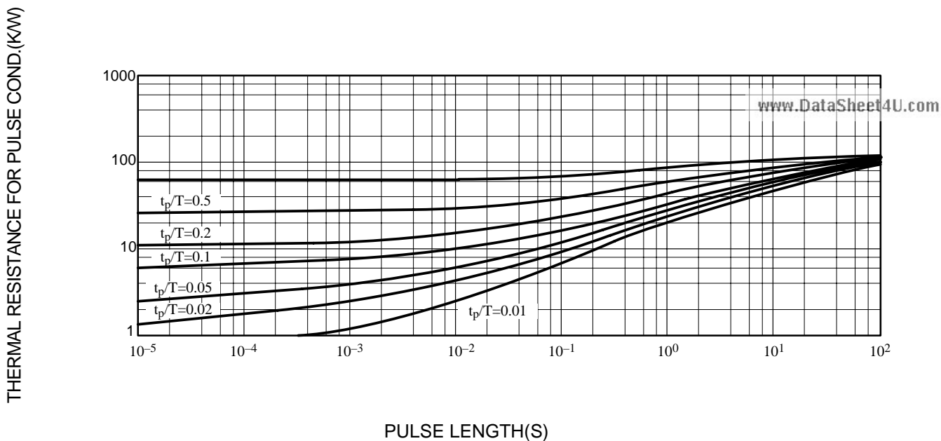
FIG.3 – THERMAL RESPONSE
