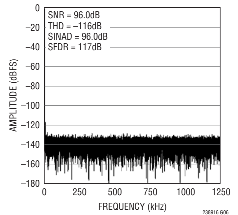
32k Point FFT f_{SMPL} = 2.5\text{Mpsps} , f_{IN} = 2\text{kHz}
