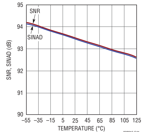
SNR, SINAD vs Temperature, f_{IN} = 2\text{kHz}
