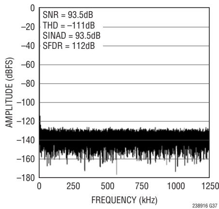
32k Point FFT f_{SAMPL} = 2.5\text{Mpsps} , f_{IN} = 2\text{kHz}
