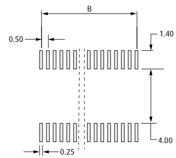
Recommended PC Board Pattern
